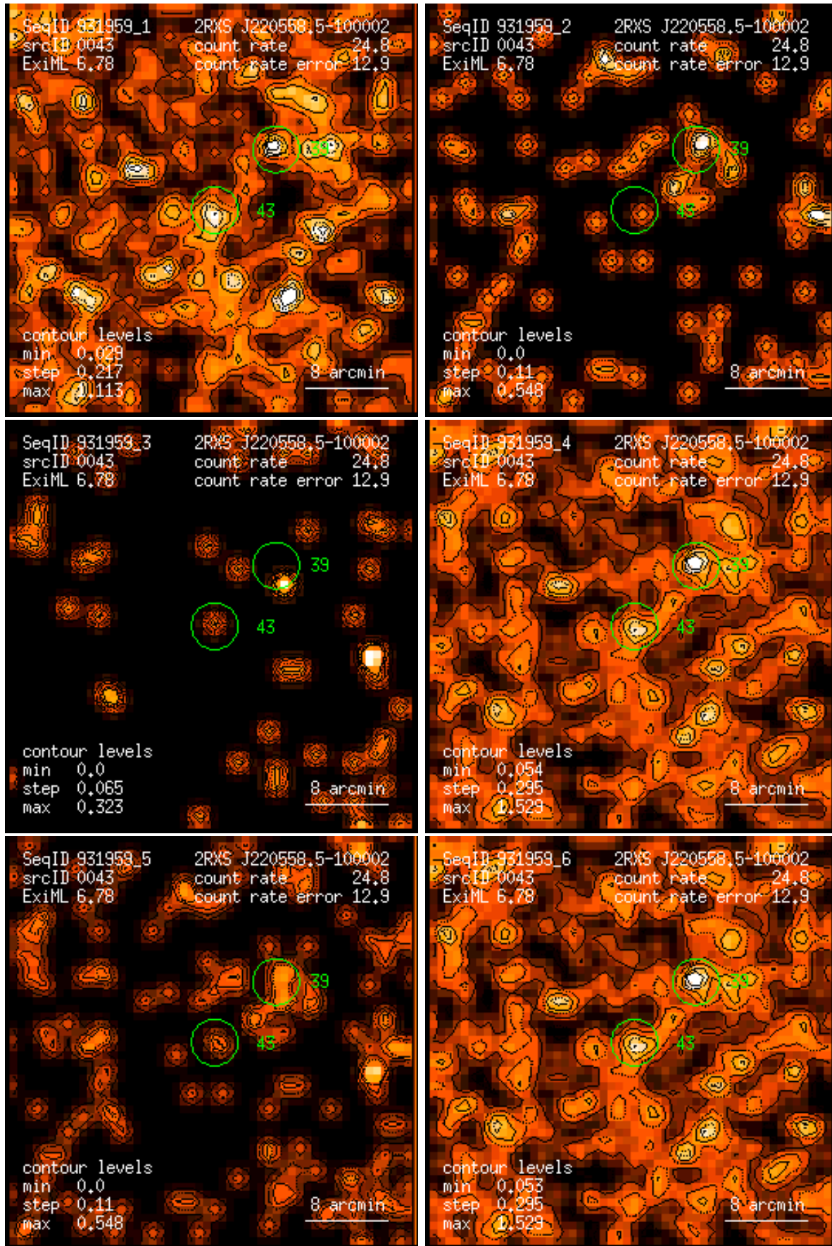
Figure 43: RASS 931959: detection 0043: band rate images, Gaussian filter: (1) PSPC channels 11 – 41, (2) 52 – 90, (3) 91 – 201, (4) 11 – 235, (5) 52 – 201, (6) 11 – 201. Broad band rates in counts/ks. Band rate contour levels in counts/ks/arcmin 2 .
