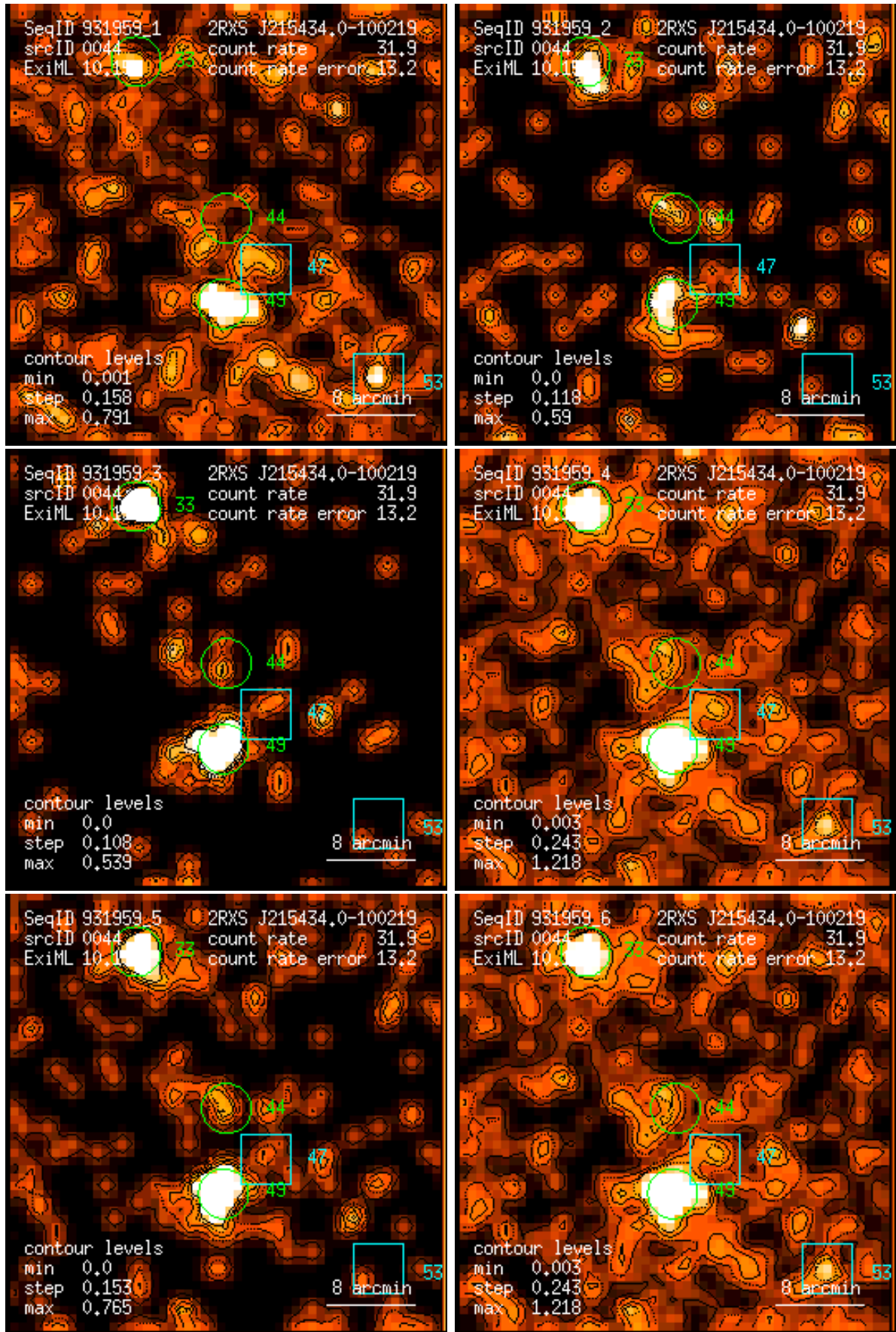
Figure 44: RASS 931959: detection 0044: band rate images, Gaussian filter: (1) PSPC channels 11 – 41, (2) 52 – 90, (3) 91 – 201, (4) 11 – 235, (5) 52 – 201, (6) 11 – 201. Broad band rates in counts/ks. Band rate contour levels in counts/ks/arcmin 2 .
