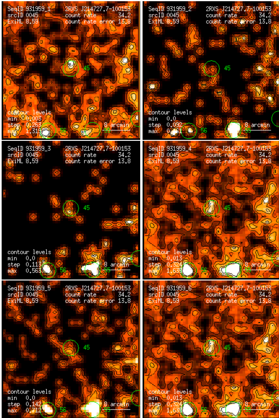
Figure 45: RASS 931959: detection 0045: band rate images, Gaussian filter: (1) PSPC channels 11 – 41, (2) 52 – 90, (3) 91 – 201, (4) 11 – 235, (5) 52 – 201, (6) 11 – 201. Broad band rates in counts/ks. Band rate contour levels in counts/ks/arcmin 2 .
