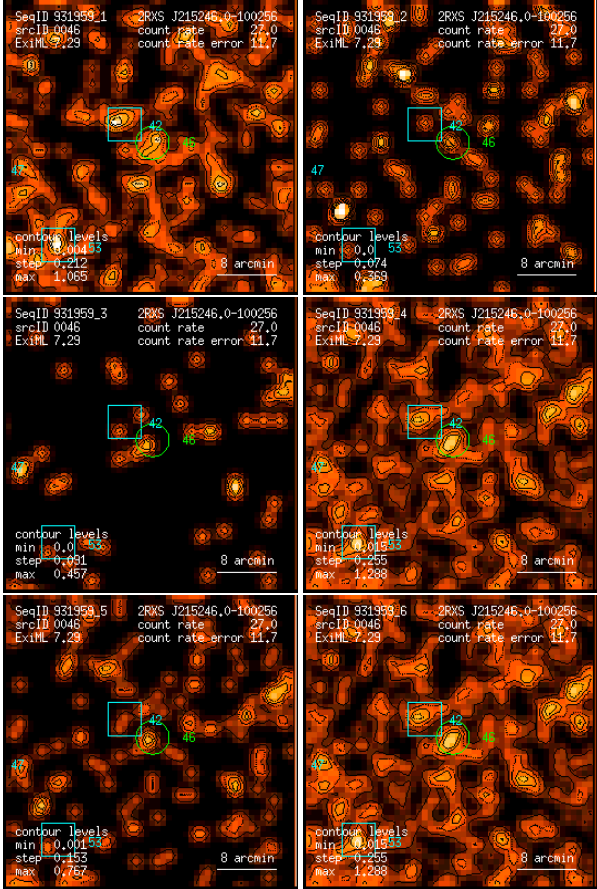
Figure 46: RASS 931959: detection 0046: band rate images, Gaussian filter: (1) PSPC channels 11 – 41, (2) 52 – 90, (3) 91 – 201, (4) 11 – 235, (5) 52 – 201, (6) 11 – 201. Broad band rates in counts/ks. Band rate contour levels in counts/ks/arcmin 2 .
