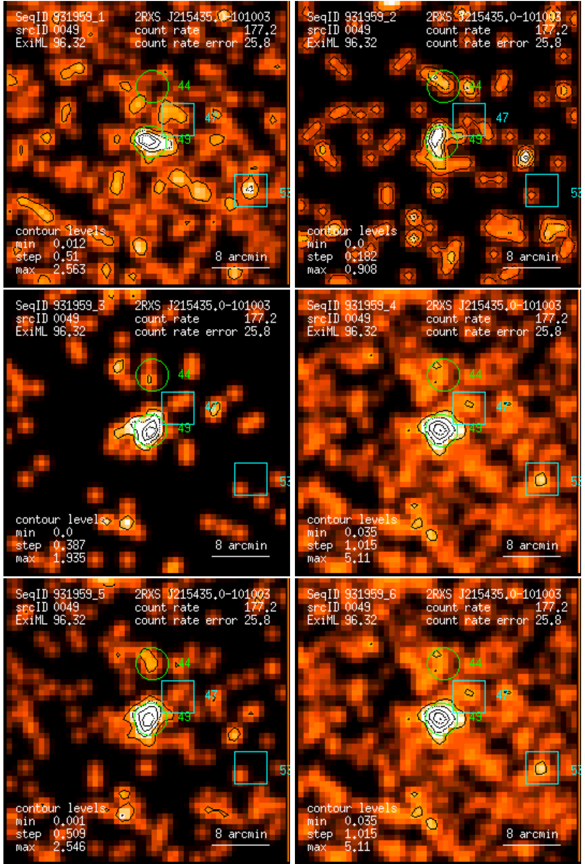
Figure 49: RASS 931959: detection 0049: band rate images, Gaussian filter: (1) PSPC channels 11 – 41, (2) 52 – 90, (3) 91 – 201, (4) 11 – 235, (5) 52 – 201, (6) 11 – 201. Broad band rates in counts/ks. Band rate contour levels in counts/ks/arcmin 2 .
