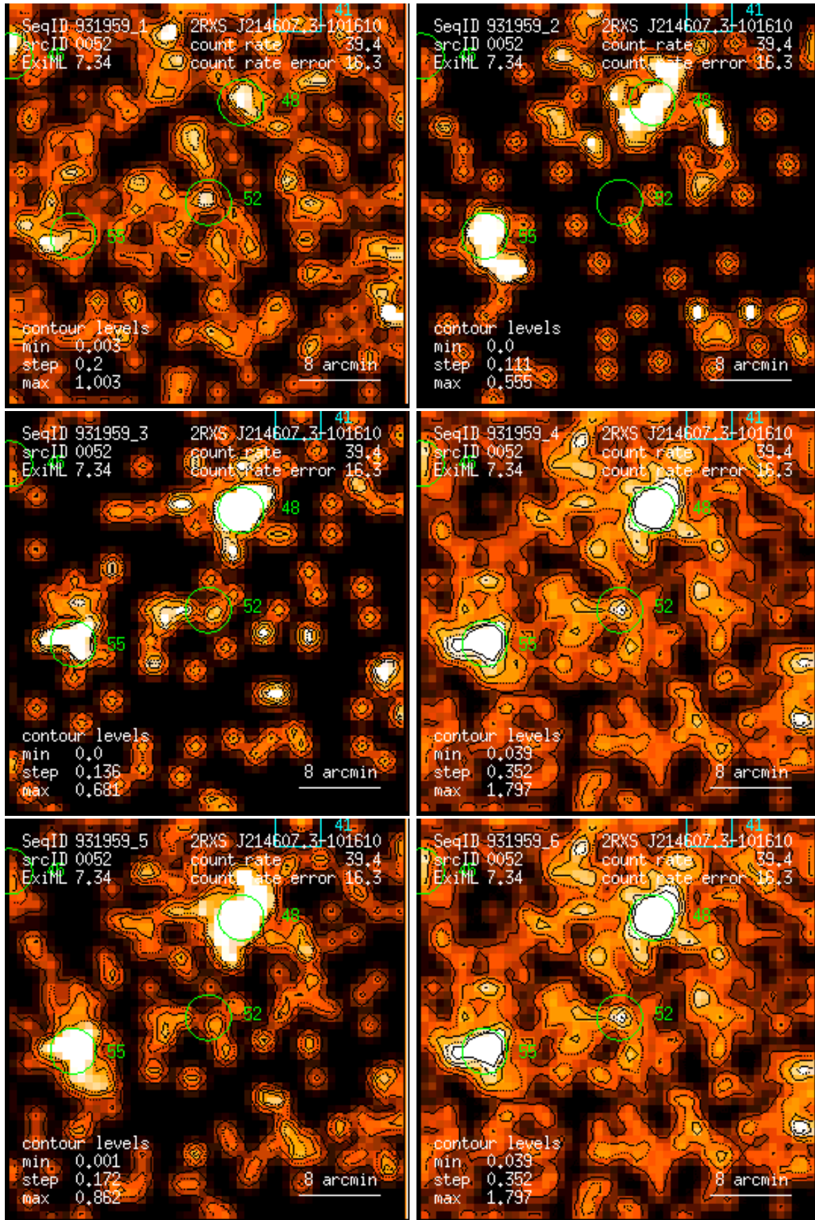
Figure 52: RASS 931959: detection 0052: band rate images, Gaussian filter: (1) PSPC channels 11 – 41, (2) 52 – 90, (3) 91 – 201, (4) 11 – 235, (5) 52 – 201, (6) 11 – 201. Broad band rates in counts/ks. Band rate contour levels in counts/ks/arcmin 2 .
