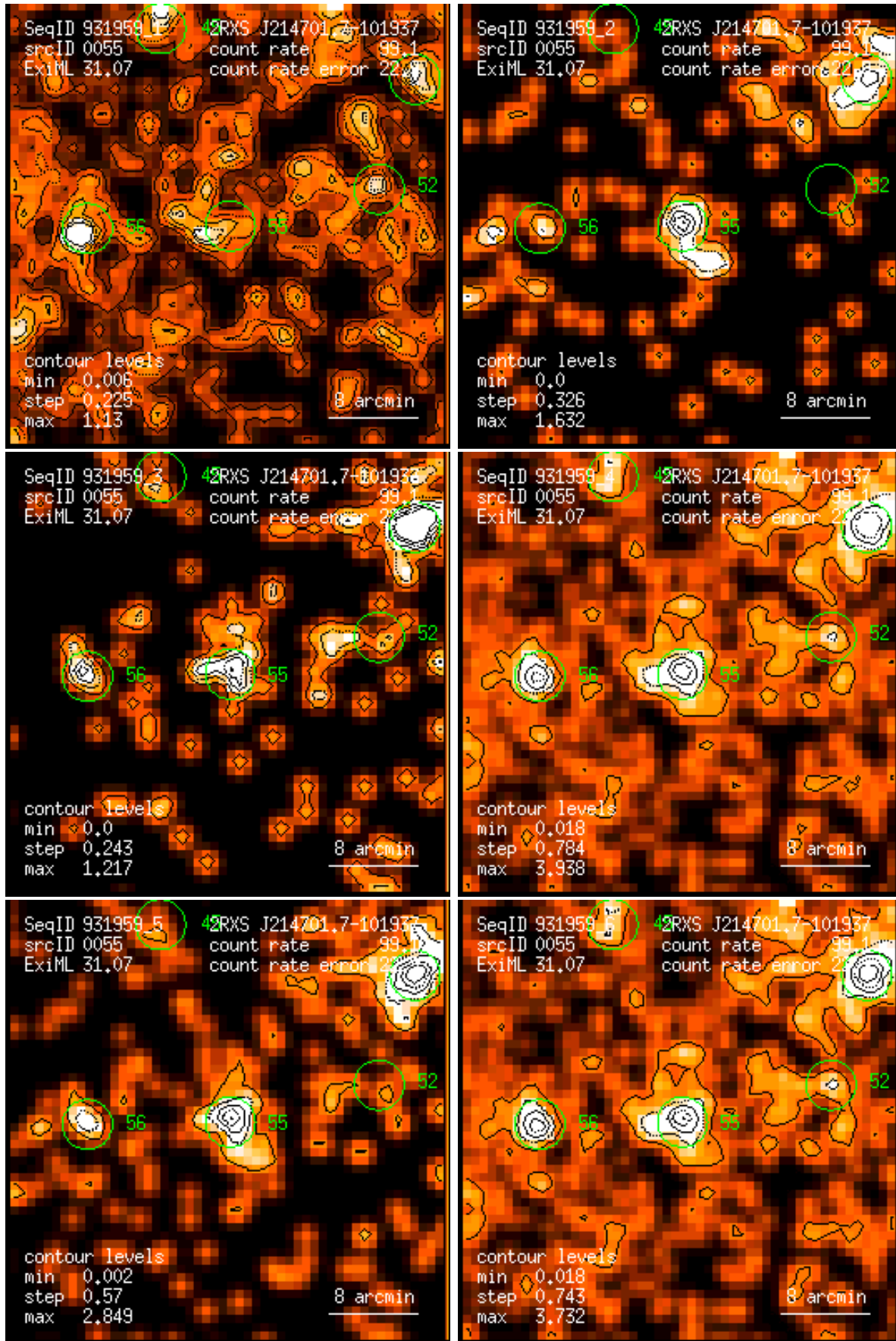
Figure 55: RASS 931959: detection 0055: band rate images, Gaussian filter: (1) PSPC channels 11 – 41, (2) 52 – 90, (3) 91 – 201, (4) 11 – 235, (5) 52 – 201, (6) 11 – 201. Broad band rates in counts/ks. Band rate contour levels in counts/ks/arcmin 2 .
