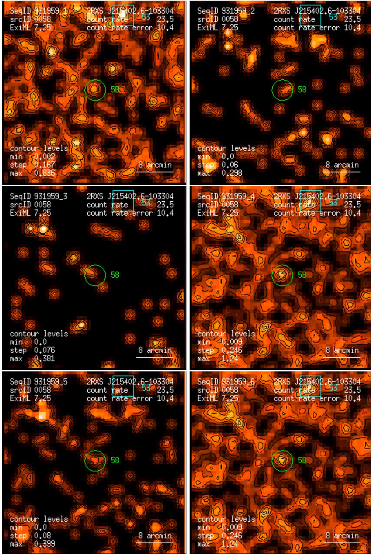
Figure 58: RASS 931959: detection 0058: band rate images, Gaussian filter: (1) PSPC channels 11 – 41, (2) 52 – 90, (3) 91 – 201, (4) 11 – 235, (5) 52 – 201, (6) 11 – 201. Broad band rates in counts/ks. Band rate contour levels in counts/ks/arcmin 2 .
