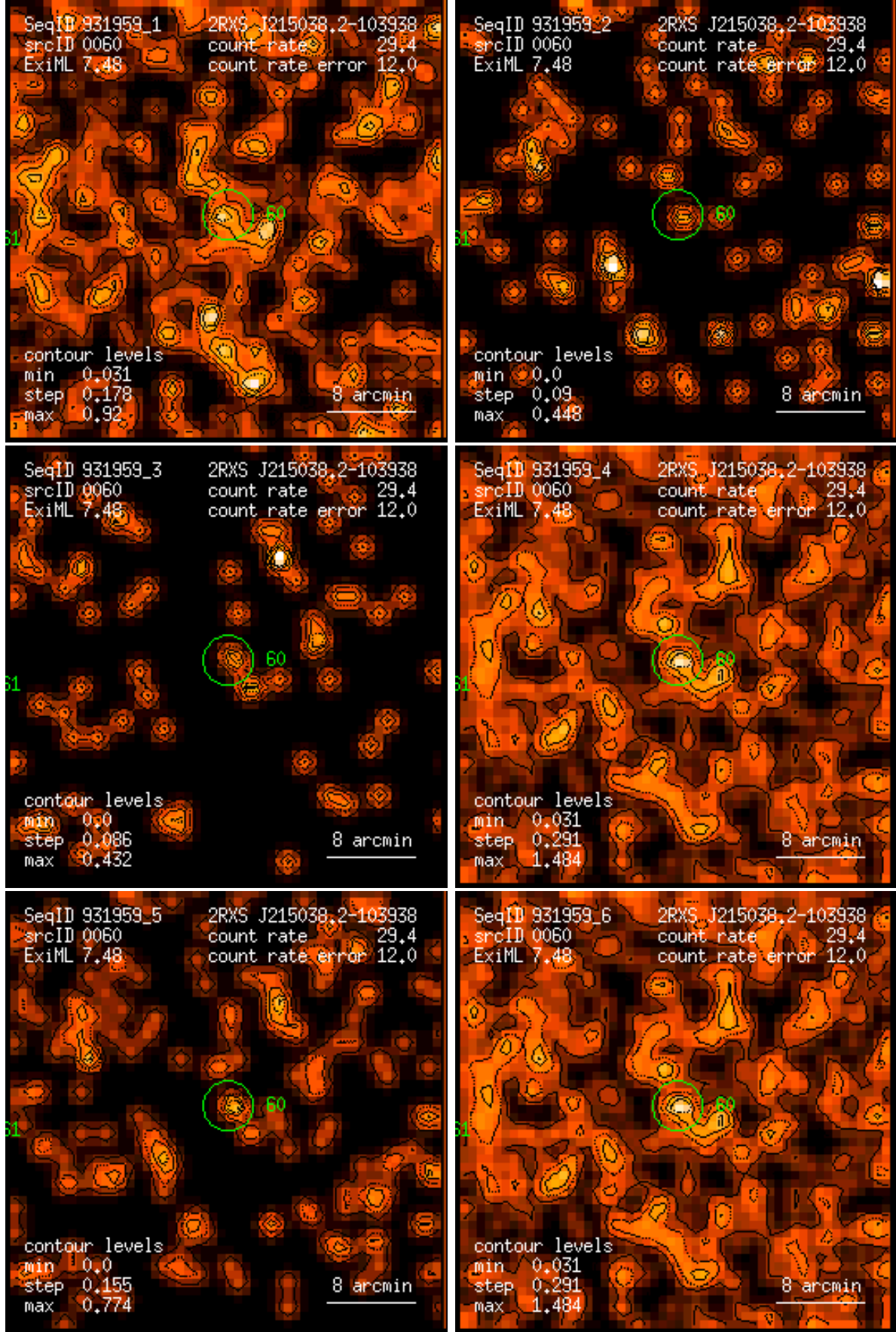
Figure 60: RASS 931959: detection 0060: band rate images, Gaussian filter: (1) PSPC channels 11 – 41, (2) 52 – 90, (3) 91 – 201, (4) 11 – 235, (5) 52 – 201, (6) 11 – 201. Broad band rates in counts/ks. Band rate contour levels in counts/ks/arcmin 2 .
