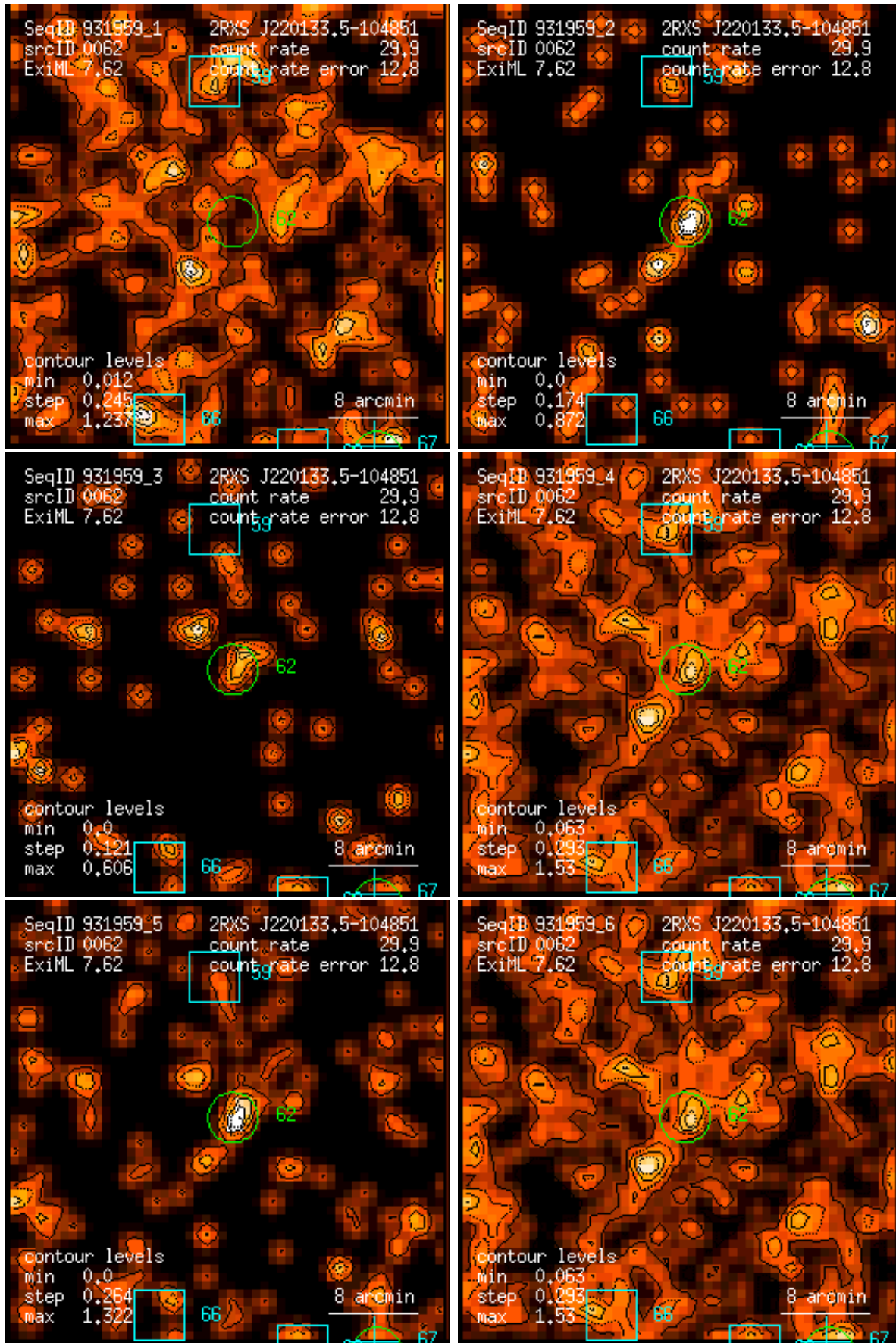
Figure 62: RASS 931959: detection 0062: band rate images, Gaussian filter: (1) PSPC channels 11 – 41, (2) 52 – 90, (3) 91 – 201, (4) 11 – 235, (5) 52 – 201, (6) 11 – 201. Broad band rates in counts/ks. Band rate contour levels in counts/ks/arcmin 2 .
