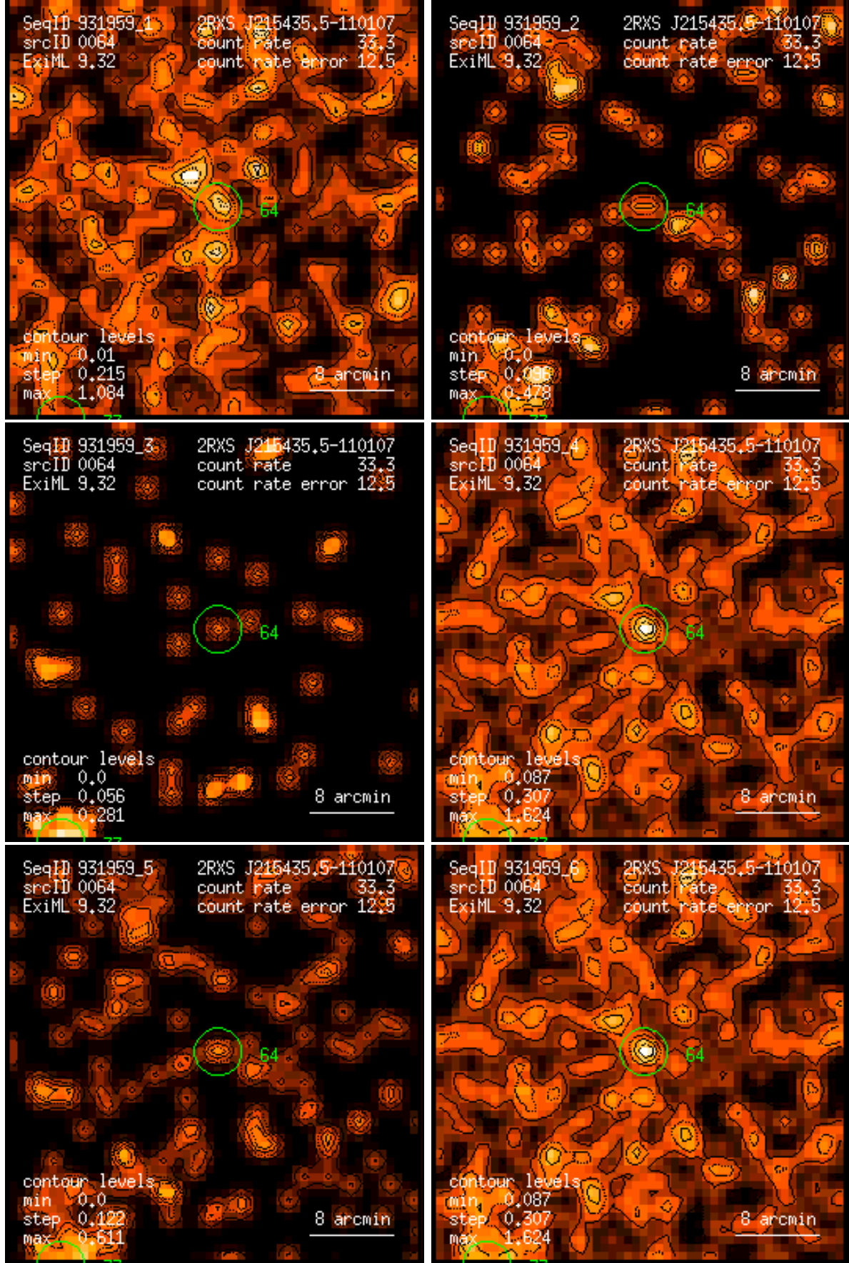
Figure 64: RASS 931959: detection 0064: band rate images, Gaussian filter: (1) PSPC channels 11 – 41, (2) 52 – 90, (3) 91 – 201, (4) 11 – 235, (5) 52 – 201, (6) 11 – 201. Broad band rates in counts/ks. Band rate contour levels in counts/ks/arcmin 2 .
