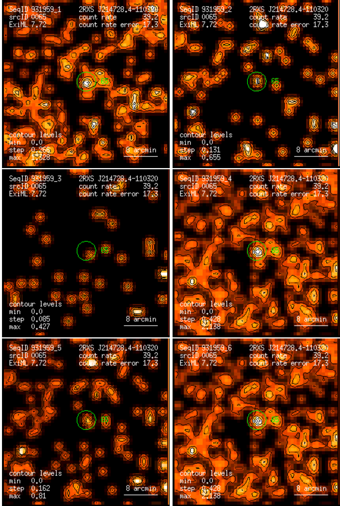
Figure 65: RASS 931959: detection 0065: band rate images, Gaussian filter: (1) PSPC channels 11 – 41, (2) 52 – 90, (3) 91 – 201, (4) 11 – 235, (5) 52 – 201, (6) 11 – 201. Broad band rates in counts/ks. Band rate contour levels in counts/ks/arcmin 2 .
