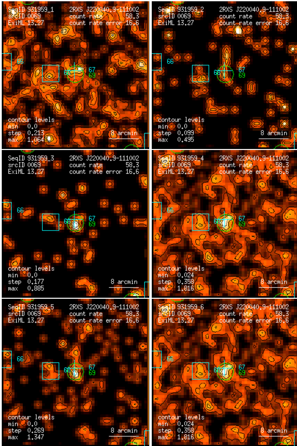
Figure 69: RASS 931959: detection 0069: band rate images, Gaussian filter: (1) PSPC channels 11 – 41, (2) 52 – 90, (3) 91 – 201, (4) 11 – 235, (5) 52 – 201, (6) 11 – 201. Broad band rates in counts/ks. Band rate contour levels in counts/ks/arcmin 2 .
