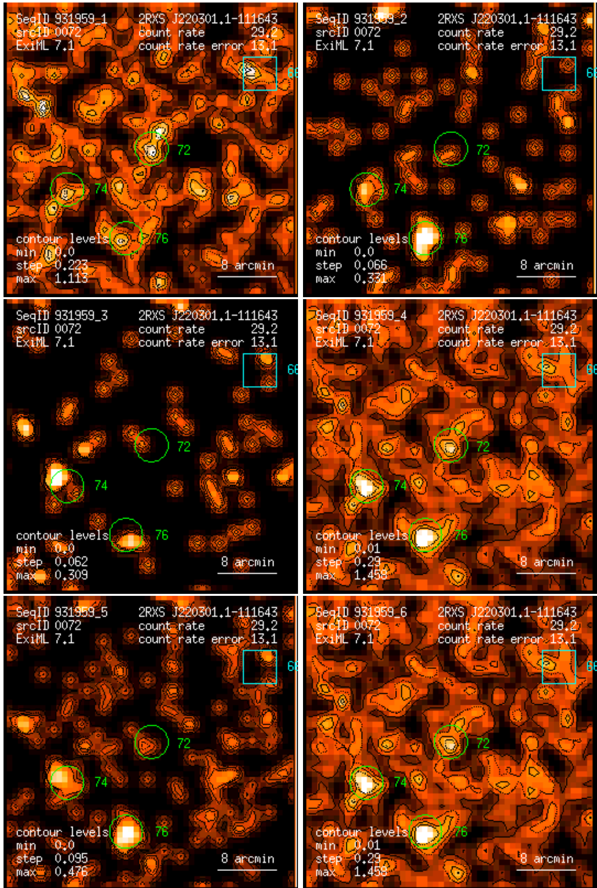
Figure 72: RASS 931959: detection 0072: band rate images, Gaussian filter: (1) PSPC channels 11 – 41, (2) 52 – 90, (3) 91 – 201, (4) 11 – 235, (5) 52 – 201, (6) 11 – 201. Broad band rates in counts/ks. Band rate contour levels in counts/ks/arcmin 2 .
