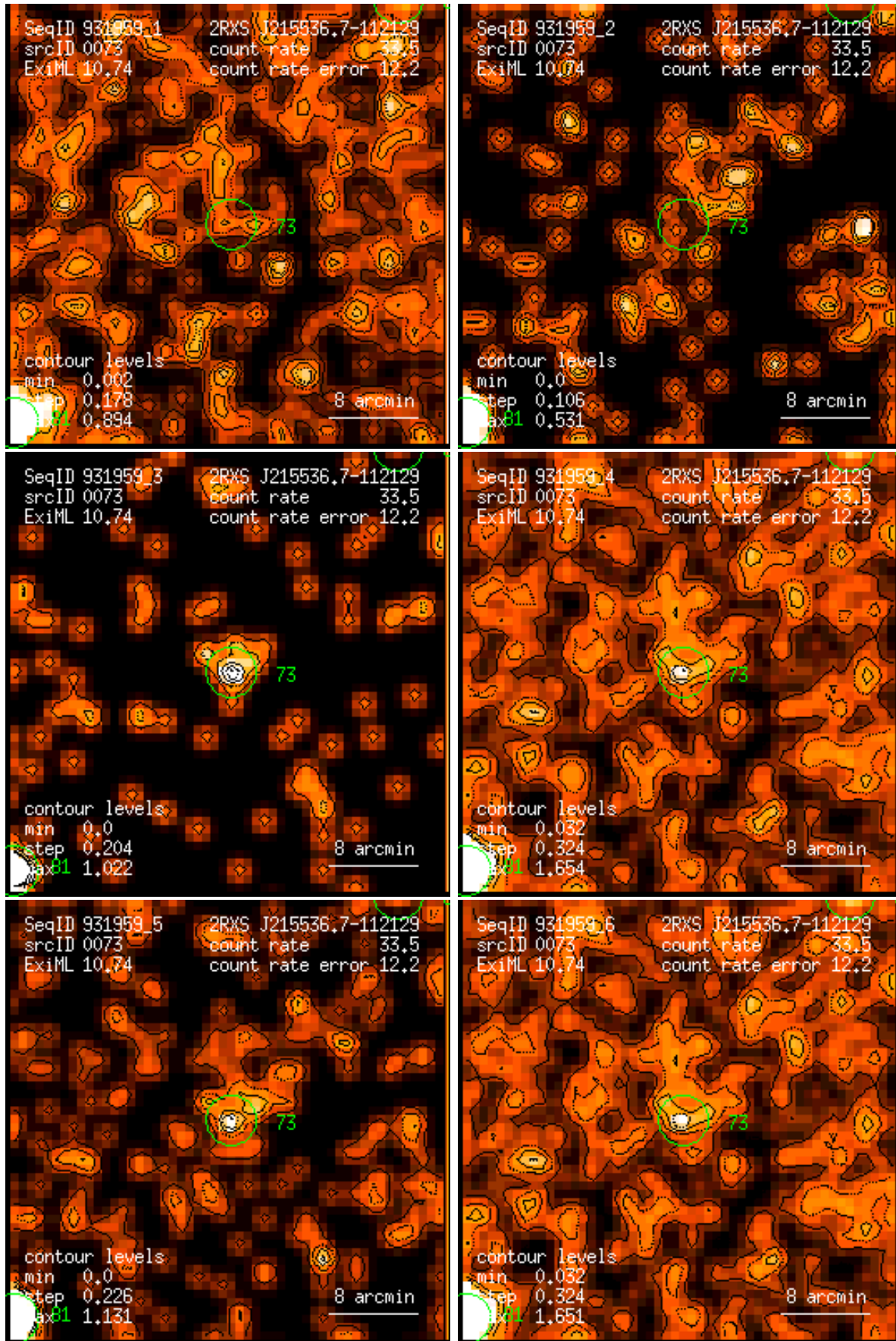
Figure 73: RASS 931959: detection 0073: band rate images, Gaussian filter: (1) PSPC channels 11 – 41, (2) 52 – 90, (3) 91 – 201, (4) 11 – 235, (5) 52 – 201, (6) 11 – 201. Broad band rates in counts/ks. Band rate contour levels in counts/ks/arcmin 2 .
