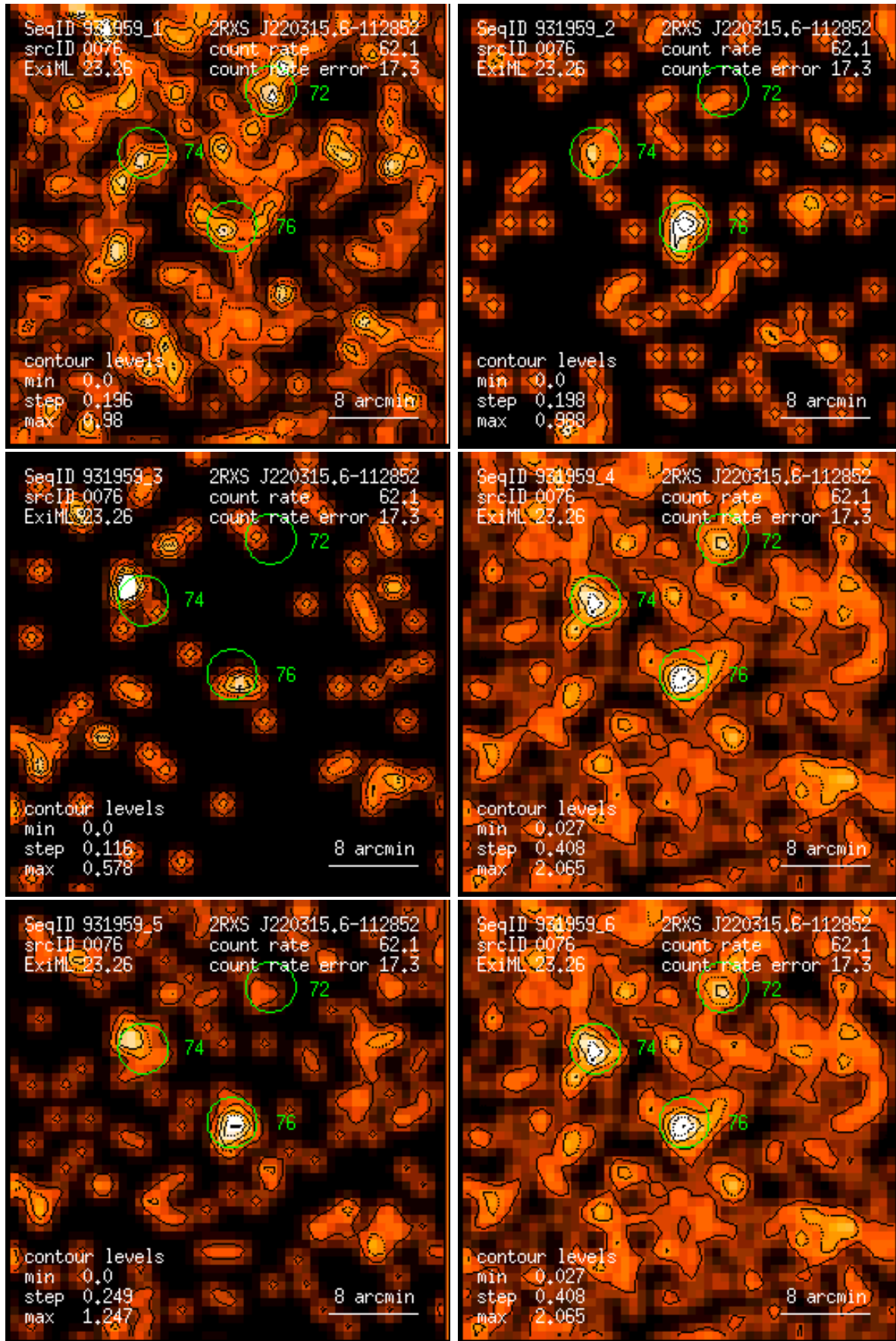
Figure 76: RASS 931959: detection 0076: band rate images, Gaussian filter: (1) PSPC channels 11 – 41, (2) 52 – 90, (3) 91 – 201, (4) 11 – 235, (5) 52 – 201, (6) 11 – 201. Broad band rates in counts/ks. Band rate contour levels in counts/ks/arcmin 2 .
