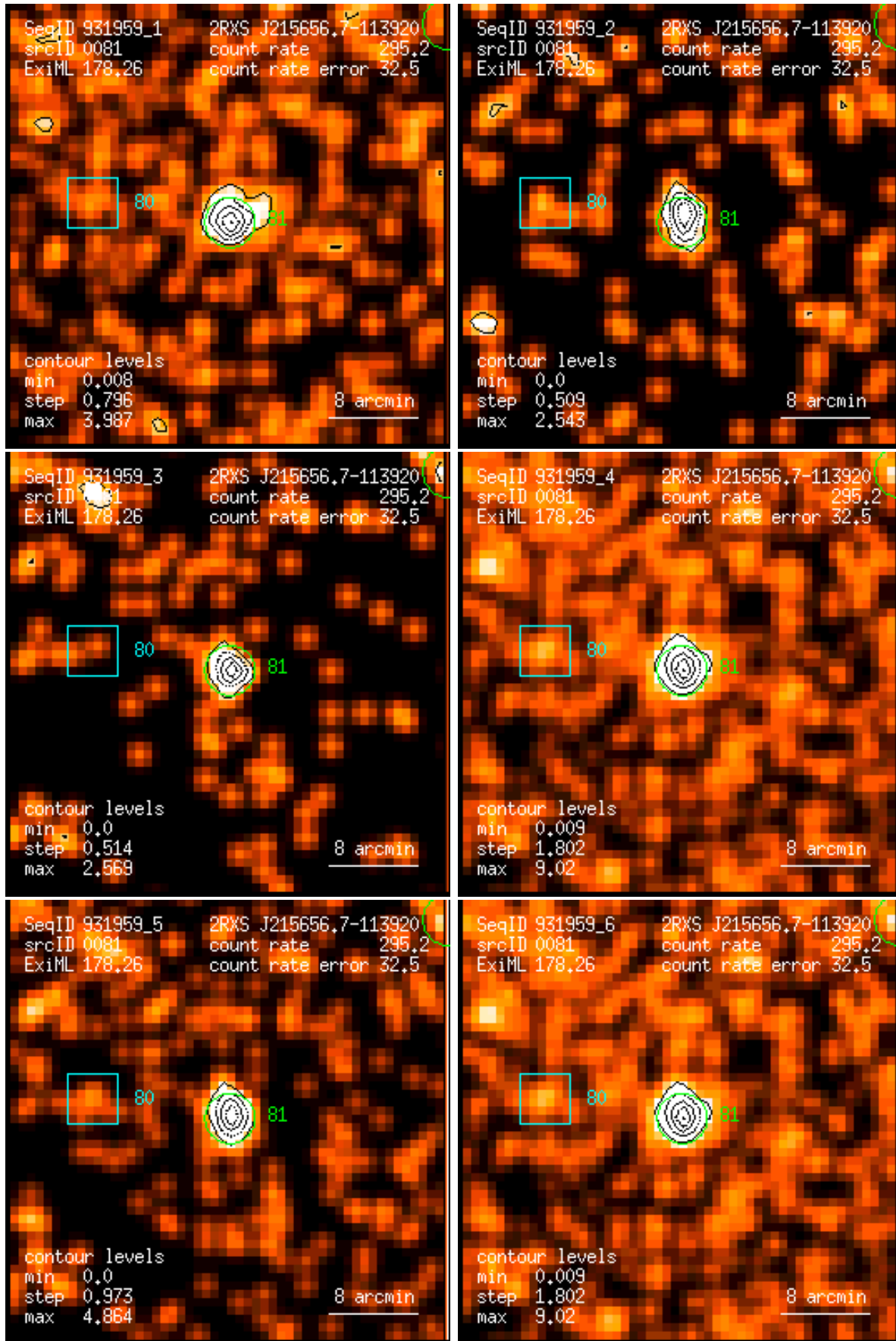
Figure 81: RASS 931959: detection 0081: band rate images, Gaussian filter: (1) PSPC channels 11 – 41, (2) 52 – 90, (3) 91 – 201, (4) 11 – 235, (5) 52 – 201, (6) 11 – 201. Broad band rates in counts/ks. Band rate contour levels in counts/ks/arcmin 2 .
