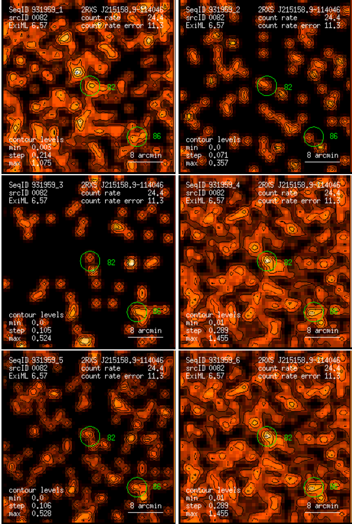
Figure 82: RASS 931959: detection 0082: band rate images, Gaussian filter: (1) PSPC channels 11 – 41, (2) 52 – 90, (3) 91 – 201, (4) 11 – 235, (5) 52 – 201, (6) 11 – 201. Broad band rates in counts/ks. Band rate contour levels in counts/ks/arcmin 2 .
