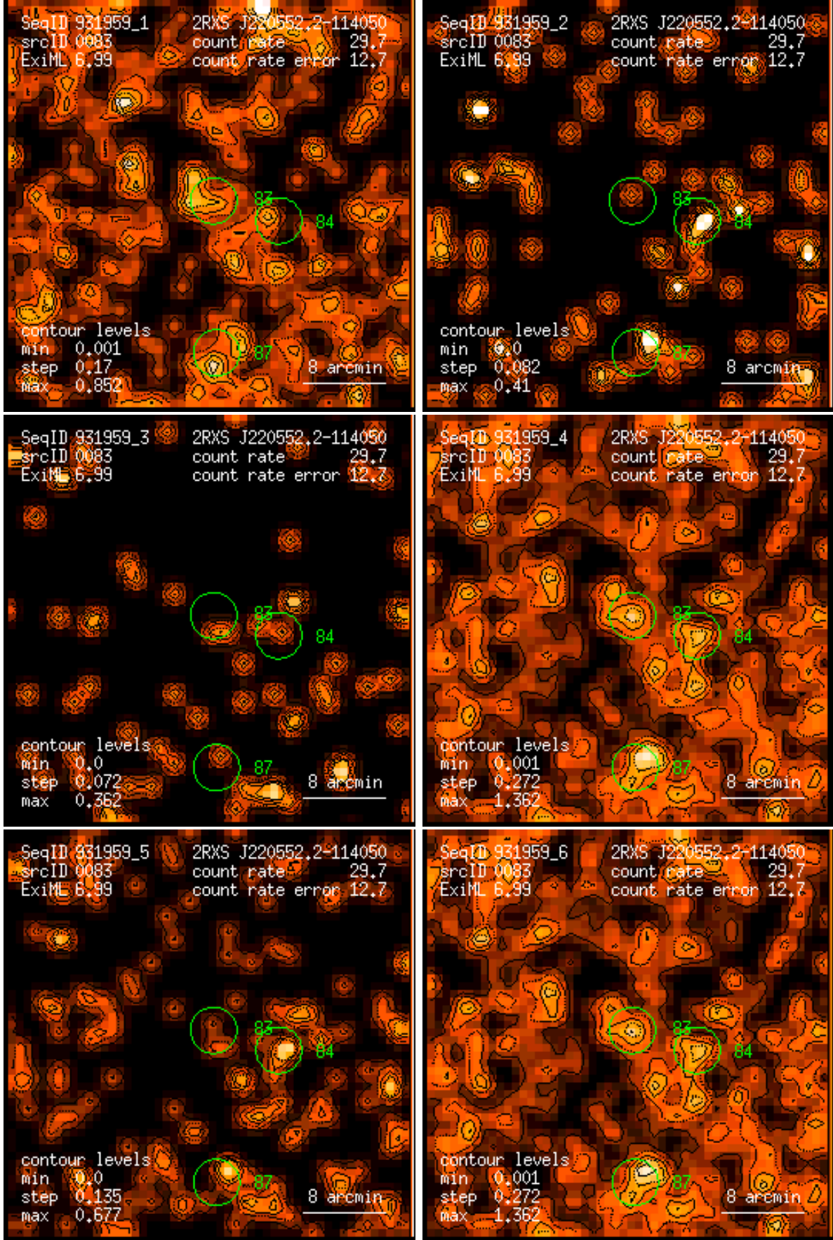
Figure 83: RASS 931959: detection 0083: band rate images, Gaussian filter: (1) PSPC channels 11 – 41, (2) 52 – 90, (3) 91 – 201, (4) 11 – 235, (5) 52 – 201, (6) 11 – 201. Broad band rates in counts/ks. Band rate contour levels in counts/ks/arcmin 2 .
