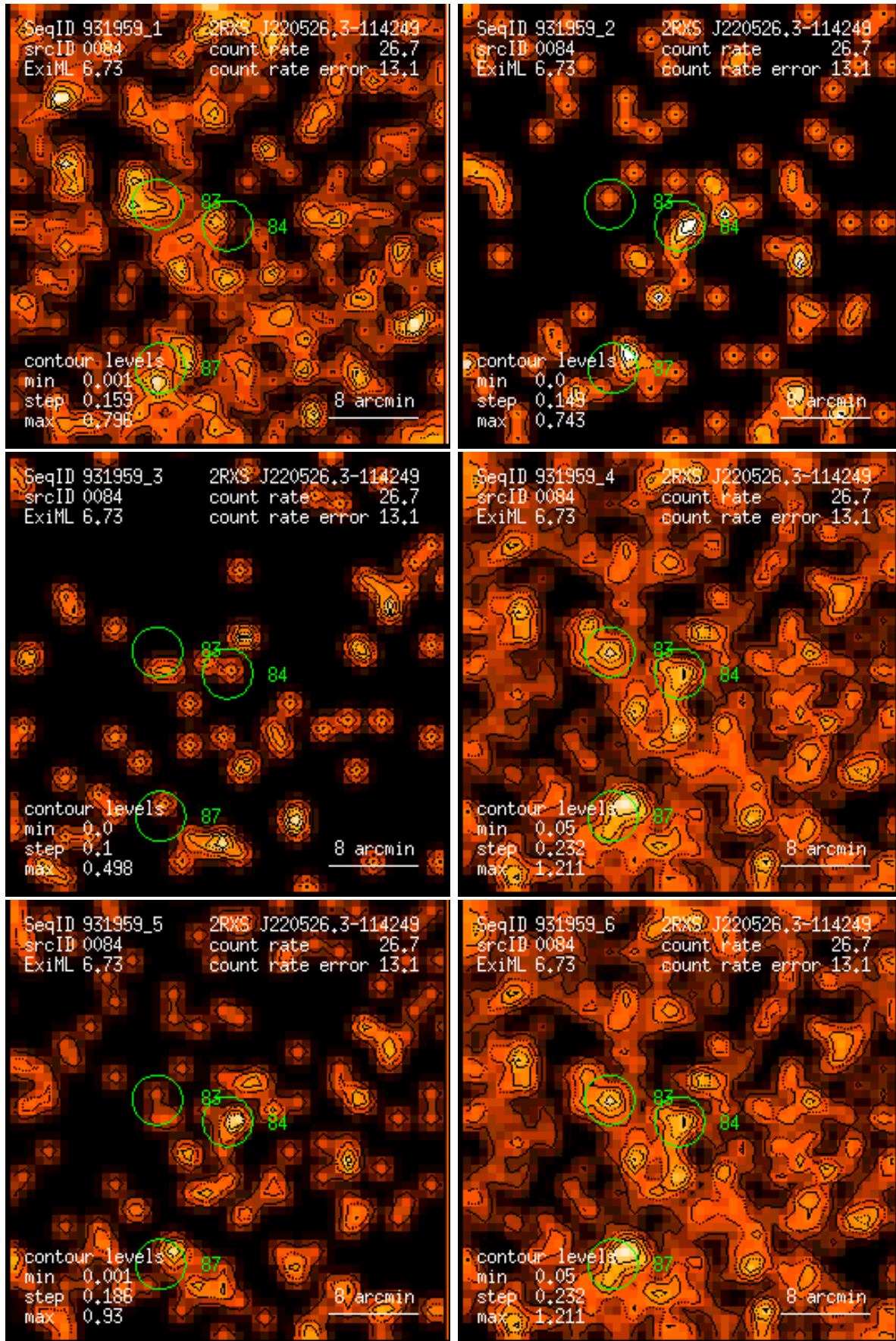
Figure 84: RASS 931959: detection 0084: band rate images, Gaussian filter: (1) PSPC channels 11 – 41, (2) 52 – 90, (3) 91 – 201, (4) 11 – 235, (5) 52 – 201, (6) 11 – 201. Broad band rates in counts/ks. Band rate contour levels in counts/ks/arcmin 2 .
