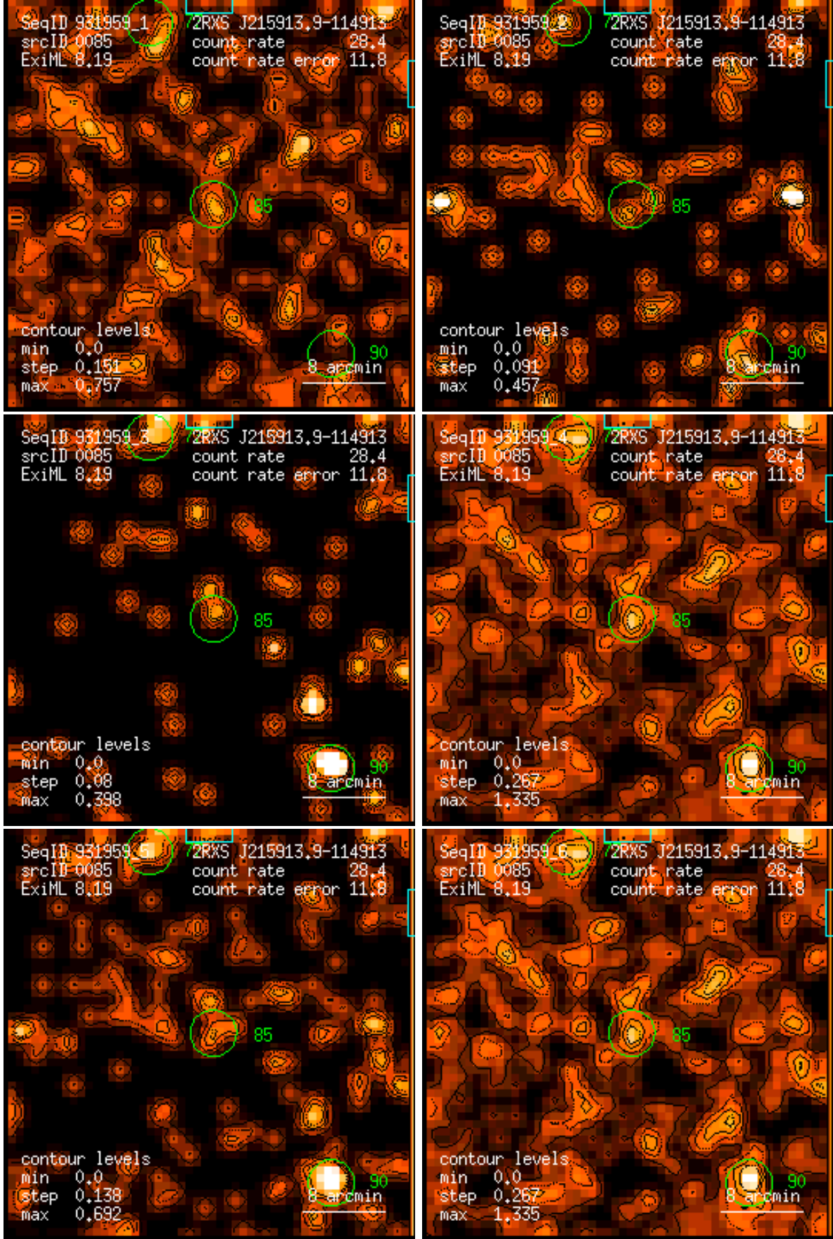
Figure 85: RASS 931959: detection 0085: band rate images, Gaussian filter: (1) PSPC channels 11 – 41, (2) 52 – 90, (3) 91 – 201, (4) 11 – 235, (5) 52 – 201, (6) 11 – 201. Broad band rates in counts/ks. Band rate contour levels in counts/ks/arcmin 2 .
