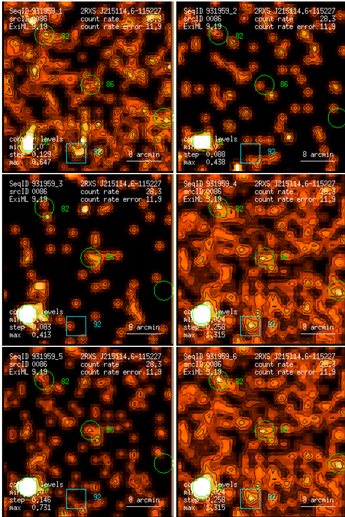
Figure 86: RASS 931959: detection 0086: band rate images, Gaussian filter: (1) PSPC channels 11 – 41, (2) 52 – 90, (3) 91 – 201, (4) 11 – 235, (5) 52 – 201, (6) 11 – 201. Broad band rates in counts/ks. Band rate contour levels in counts/ks/arcmin 2 .
