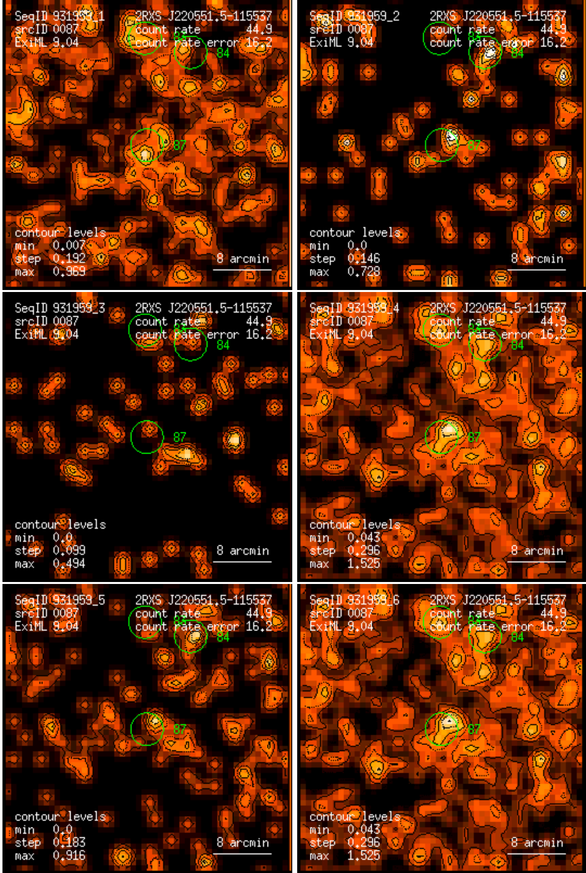
Figure 87: RASS 931959: detection 0087: band rate images, Gaussian filter: (1) PSPC channels 11 – 41, (2) 52 – 90, (3) 91 – 201, (4) 11 – 235, (5) 52 – 201, (6) 11 – 201. Broad band rates in counts/ks. Band rate contour levels in counts/ks/arcmin 2 .
