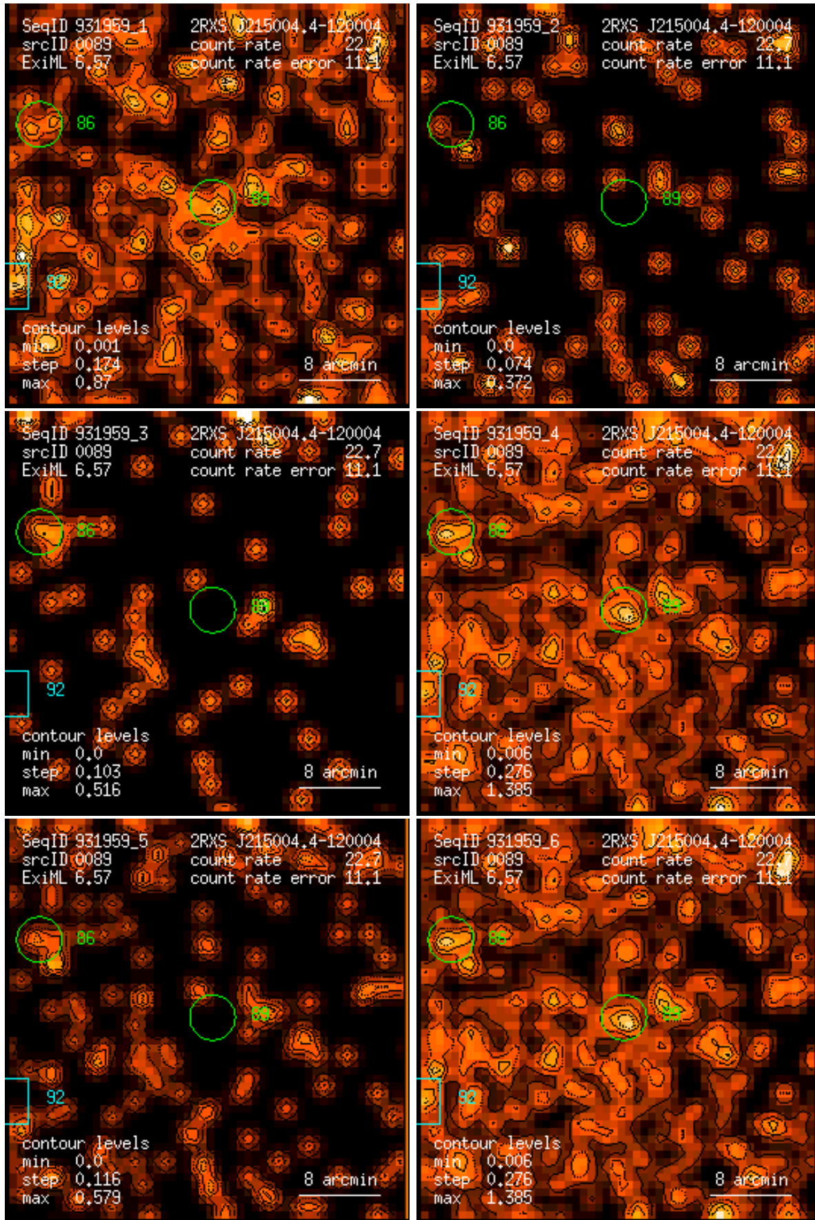
Figure 89: RASS 931959: detection 0089: band rate images, Gaussian filter: (1) PSPC channels 11 – 41, (2) 52 – 90, (3) 91 – 201, (4) 11 – 235, (5) 52 – 201, (6) 11 – 201. Broad band rates in counts/ks. Band rate contour levels in counts/ks/arcmin 2 .
