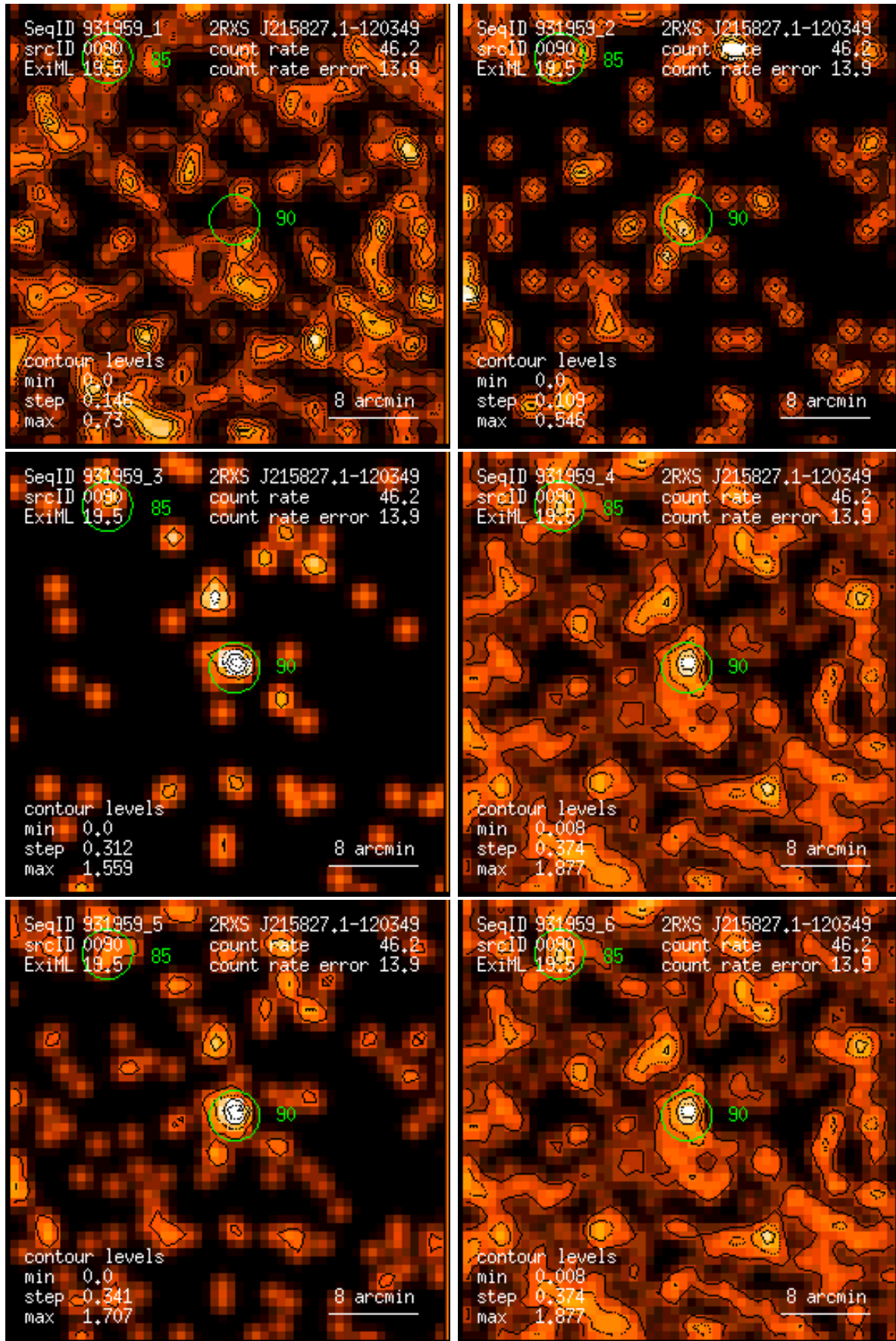
Figure 90: RASS 931959: detection 0090: band rate images, Gaussian filter: (1) PSPC channels 11 – 41, (2) 52 – 90, (3) 91 – 201, (4) 11 – 235, (5) 52 – 201, (6) 11 – 201. Broad band rates in counts/ks. Band rate contour levels in counts/ks/arcmin 2 .
