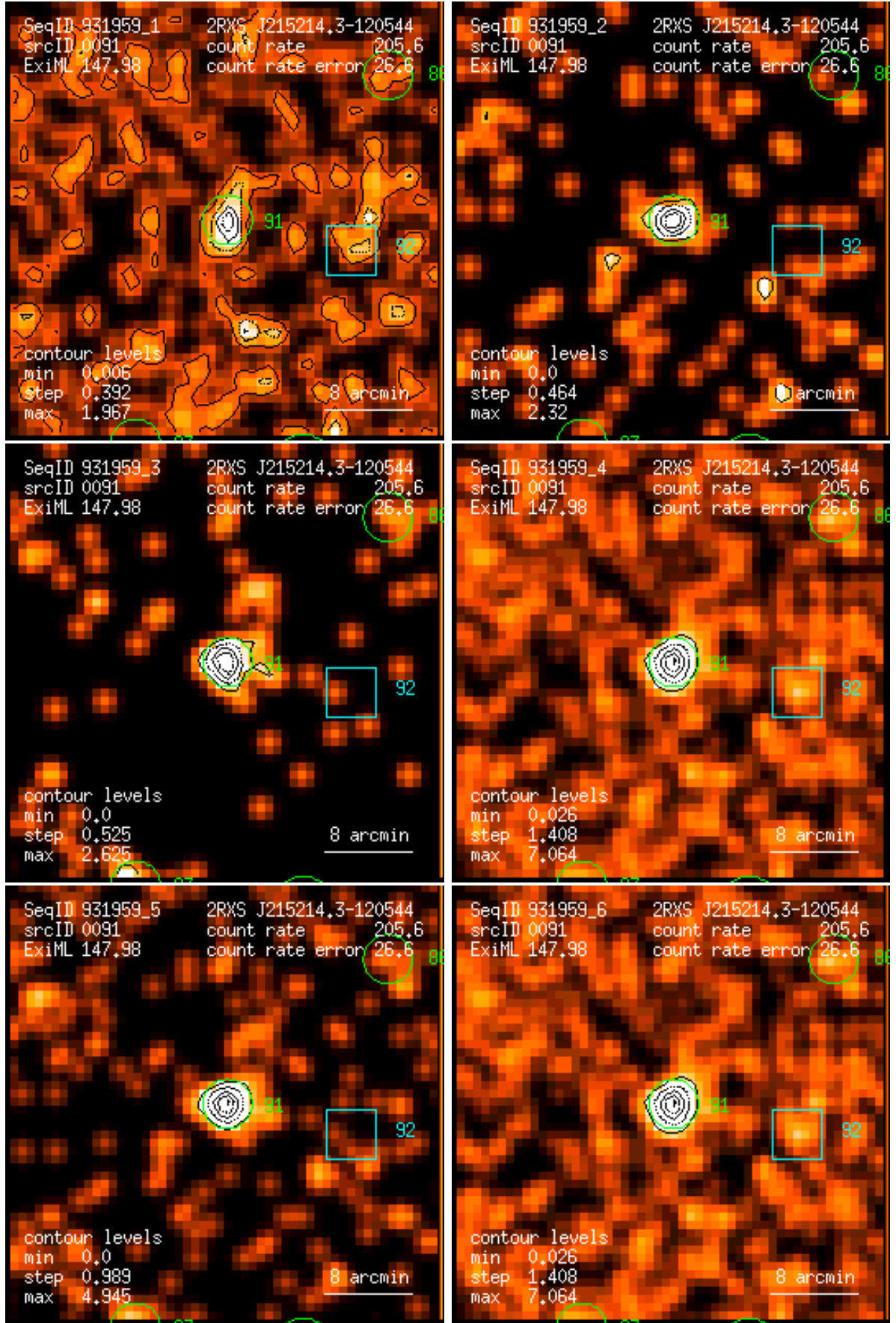
Figure 91: RASS 931959: detection 0091: band rate images, Gaussian filter: (1) PSPC channels 11 – 41, (2) 52 – 90, (3) 91 – 201, (4) 11 – 235, (5) 52 – 201, (6) 11 – 201. Broad band rates in counts/ks. Band rate contour levels in counts/ks/arcmin 2 .
