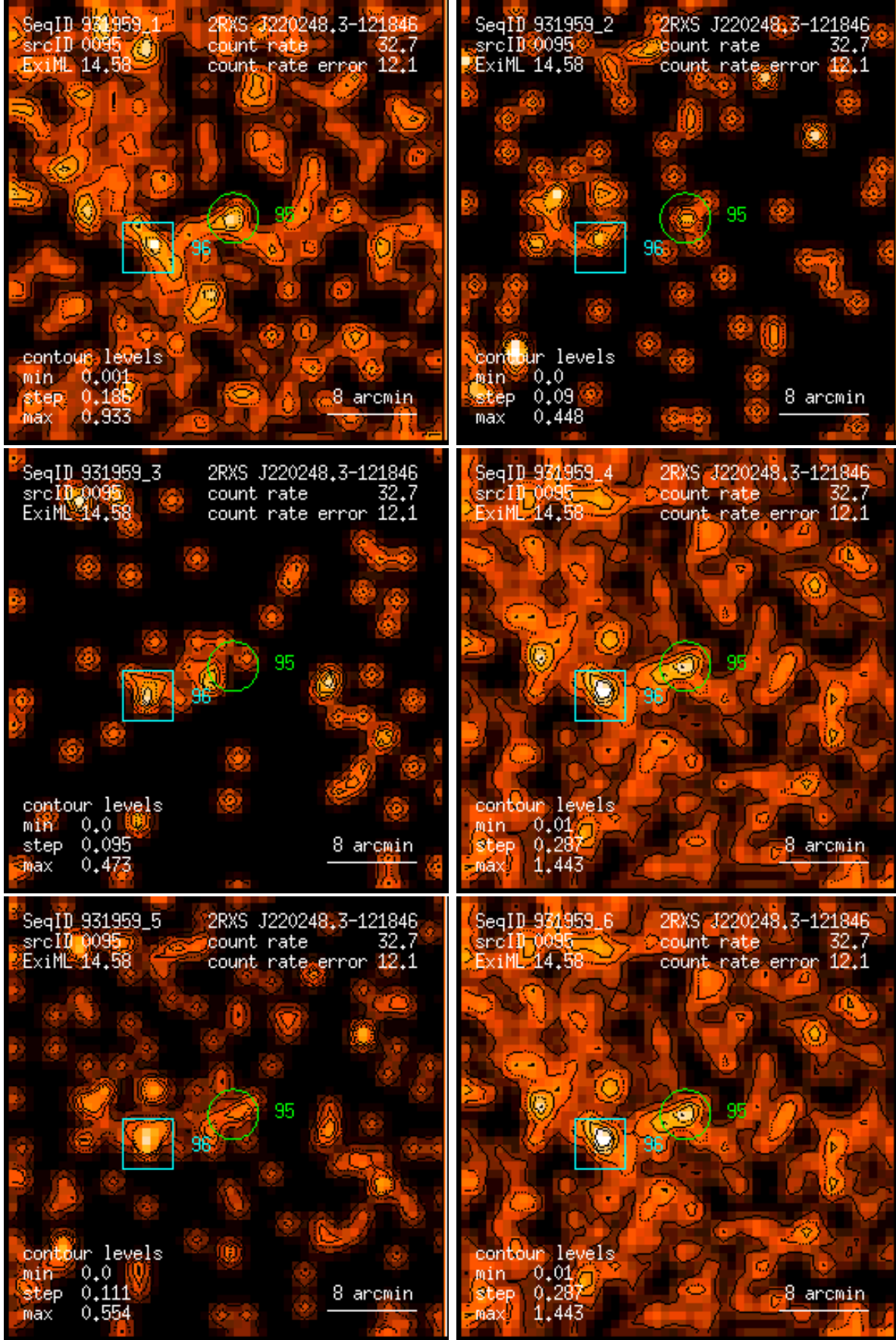
Figure 95: RASS 931959: detection 0095: band rate images, Gaussian filter: (1) PSPC channels 11 – 41, (2) 52 – 90, (3) 91 – 201, (4) 11 – 235, (5) 52 – 201, (6) 11 – 201. Broad band rates in counts/ks. Band rate contour levels in counts/ks/arcmin 2 .
