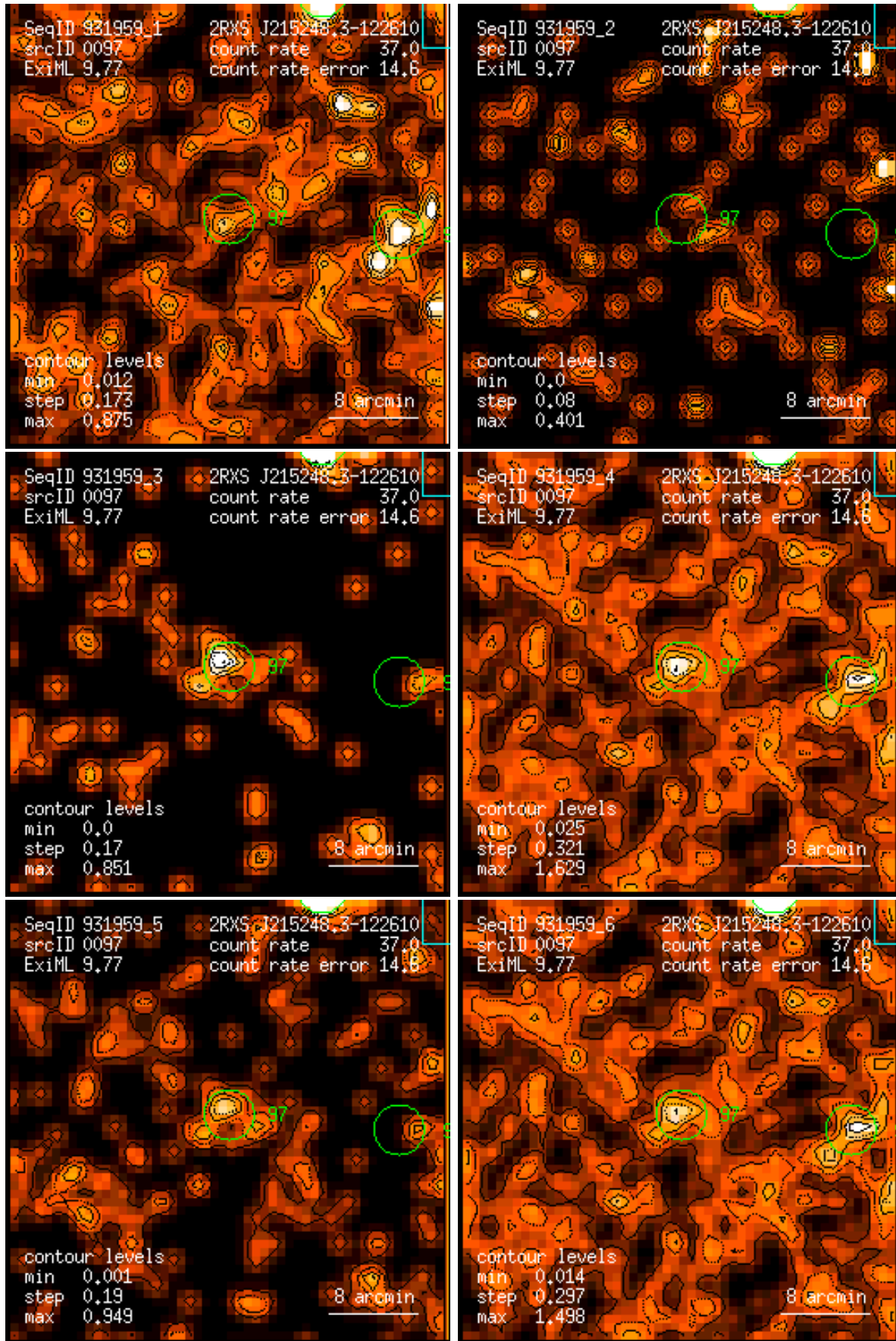
Figure 97: RASS 931959: detection 0097: band rate images, Gaussian filter: (1) PSPC channels 11 – 41, (2) 52 – 90, (3) 91 – 201, (4) 11 – 235, (5) 52 – 201, (6) 11 – 201. Broad band rates in counts/ks. Band rate contour levels in counts/ks/arcmin 2 .
