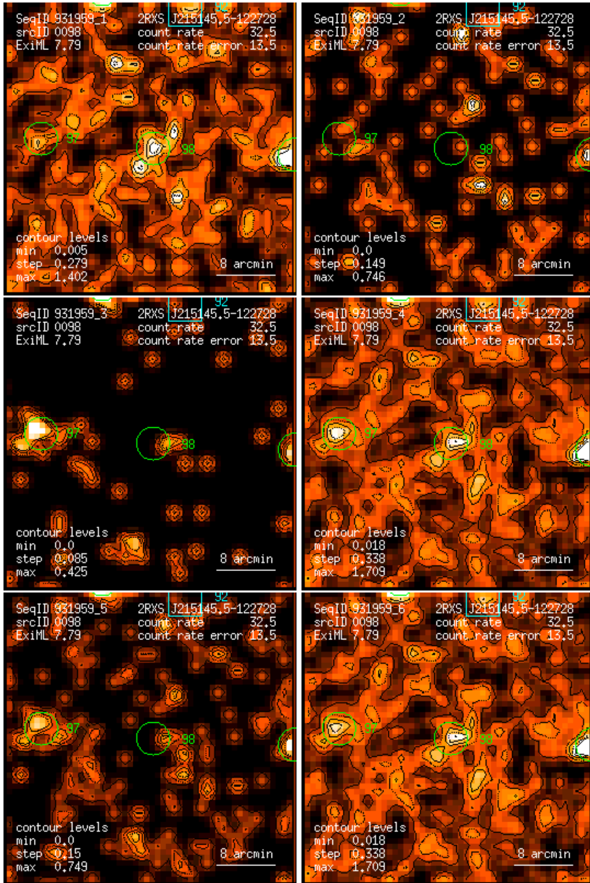
Figure 98: RASS 931959: detection 0098: band rate images, Gaussian filter: (1) PSPC channels 11 – 41, (2) 52 – 90, (3) 91 – 201, (4) 11 – 235, (5) 52 – 201, (6) 11 – 201. Broad band rates in counts/ks. Band rate contour levels in counts/ks/arcmin 2 .
