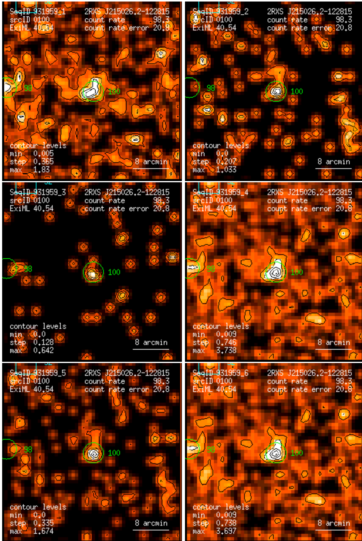
Figure 100: RASS 931959: detection 0100: band rate images, Gaussian filter: (1) PSPC channels 11 – 41, (2) 52 – 90, (3) 91 – 201, (4) 11 – 235, (5) 52 – 201, (6) 11 – 201. Broad band rates in counts/ks. Band rate contour levels in counts/ks/arcmin 2 .
