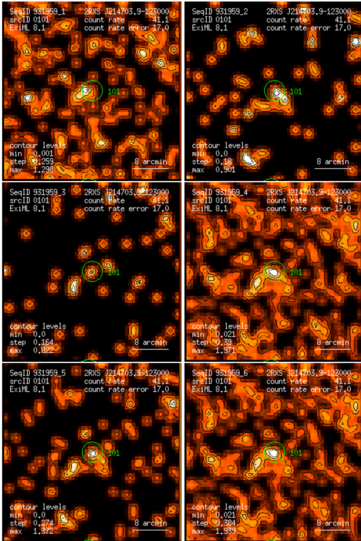
Figure 101: RASS 931959: detection 0101: band rate images, Gaussian filter: (1) PSPC channels 11 – 41, (2) 52 – 90, (3) 91 – 201, (4) 11 – 235, (5) 52 – 201, (6) 11 – 201. Broad band rates in counts/ks. Band rate contour levels in counts/ks/arcmin 2 .
