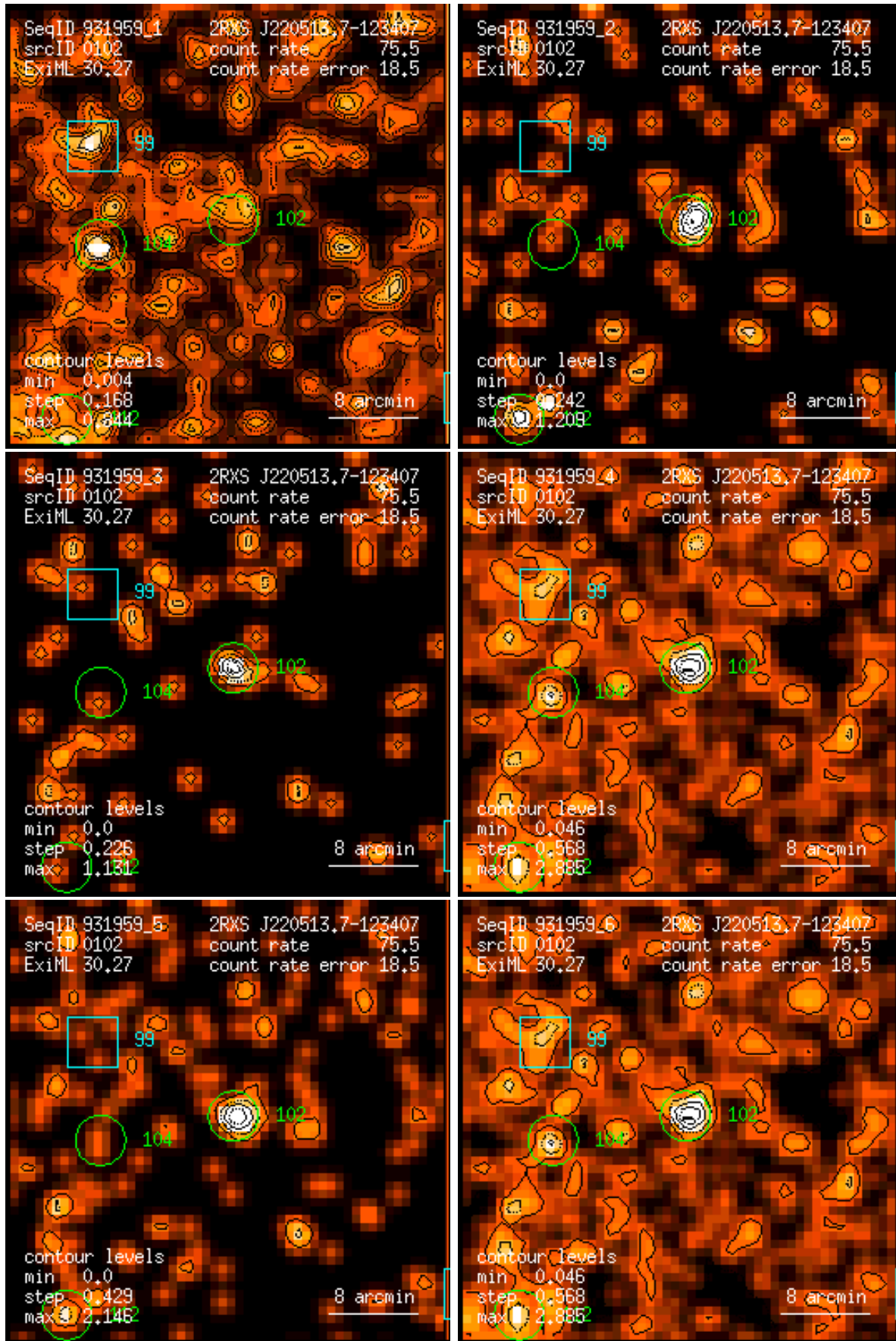
Figure 102: RASS 931959: detection 0102: band rate images, Gaussian filter: (1) PSPC channels 11 – 41, (2) 52 – 90, (3) 91 – 201, (4) 11 – 235, (5) 52 – 201, (6) 11 – 201. Broad band rates in counts/ks. Band rate contour levels in counts/ks/arcmin 2 .
