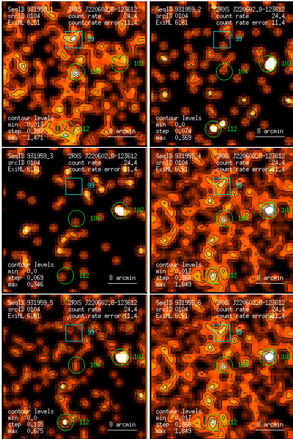
Figure 104: RASS 931959: detection 0104: band rate images, Gaussian filter: (1) PSPC channels 11 – 41, (2) 52 – 90, (3) 91 – 201, (4) 11 – 235, (5) 52 – 201, (6) 11 – 201. Broad band rates in counts/ks. Band rate contour levels in counts/ks/arcmin 2 .
