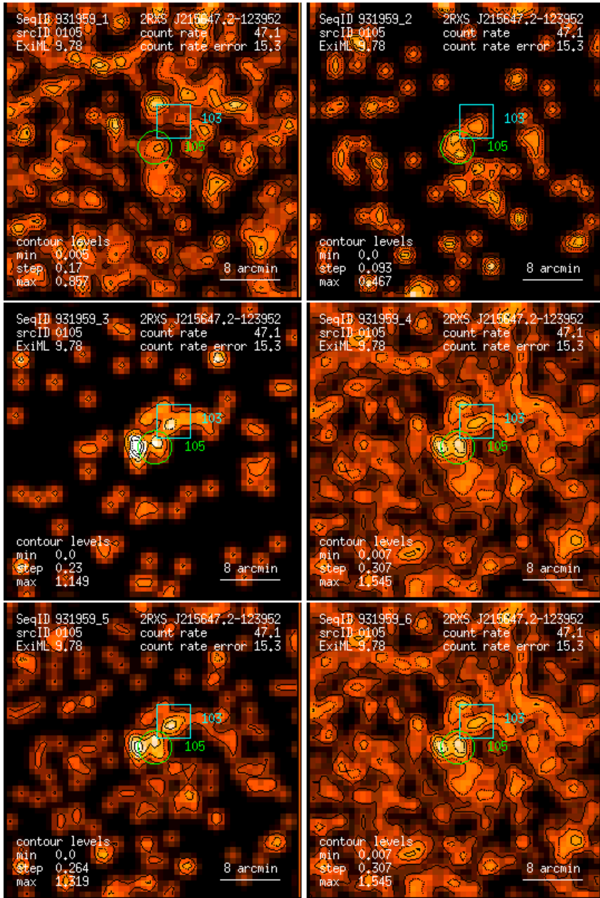
Figure 105: RASS 931959: detection 0105: band rate images, Gaussian filter: (1) PSPC channels 11 – 41, (2) 52 – 90, (3) 91 – 201, (4) 11 – 235, (5) 52 – 201, (6) 11 – 201. Broad band rates in counts/ks. Band rate contour levels in counts/ks/arcmin 2 .
