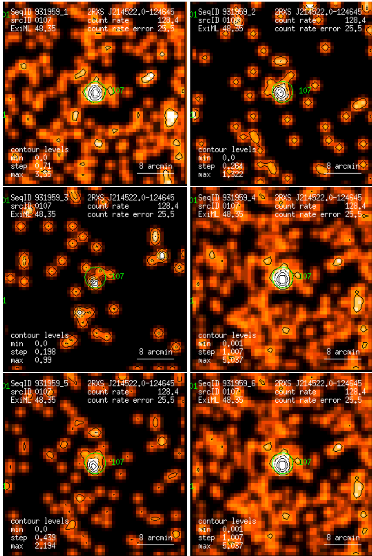
Figure 107: RASS 931959: detection 0107: band rate images, Gaussian filter: (1) PSPC channels 11 – 41, (2) 52 – 90, (3) 91 – 201, (4) 11 – 235, (5) 52 – 201, (6) 11 – 201. Broad band rates in counts/ks. Band rate contour levels in counts/ks/arcmin 2 .
