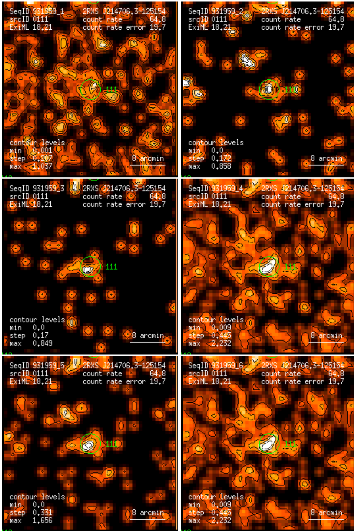
Figure 111: RASS 931959: detection 0111: band rate images, Gaussian filter: (1) PSPC channels 11 – 41, (2) 52 – 90, (3) 91 – 201, (4) 11 – 235, (5) 52 – 201, (6) 11 – 201. Broad band rates in counts/ks. Band rate contour levels in counts/ks/arcmin 2 .
