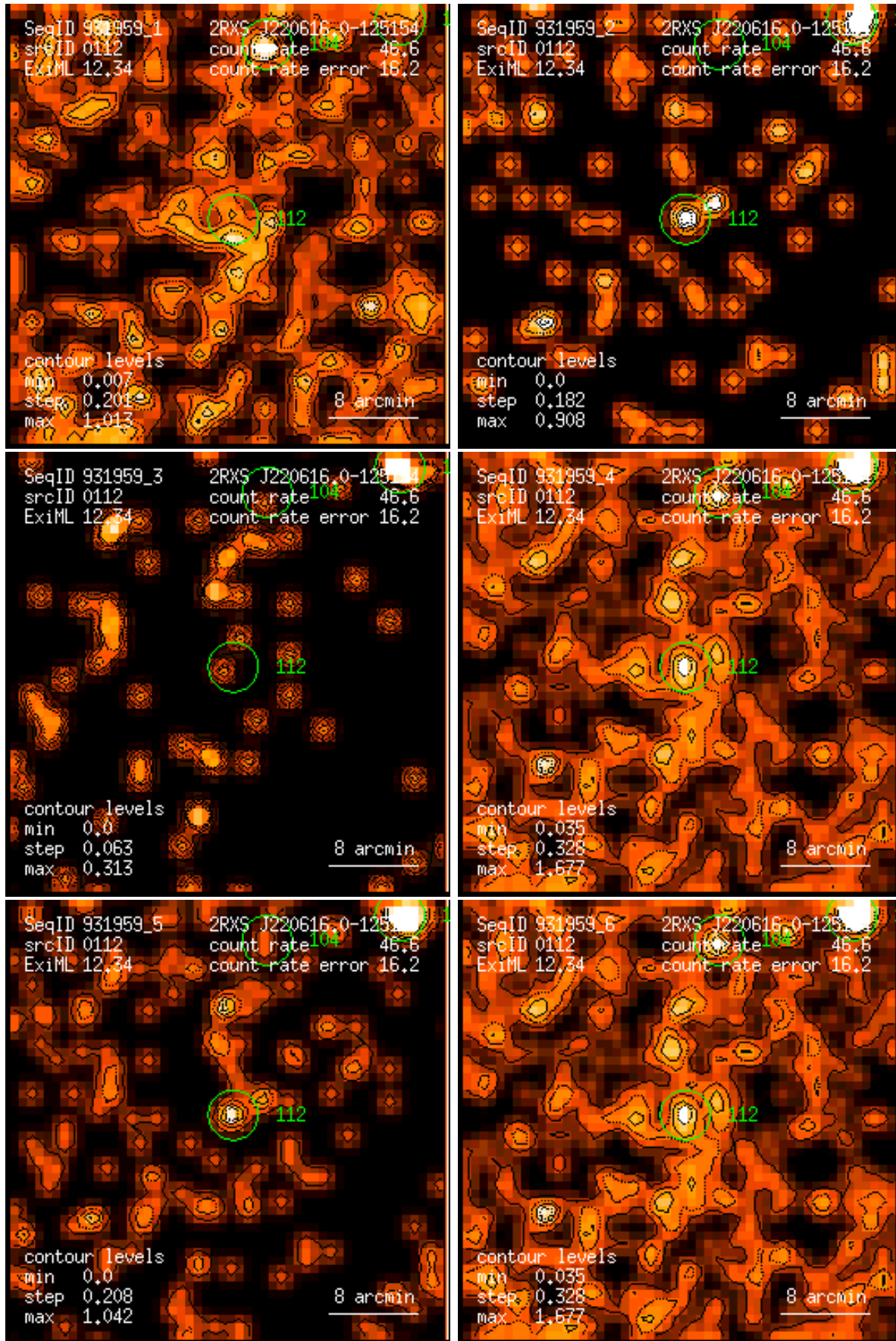
Figure 112: RASS 931959: detection 0112: band rate images, Gaussian filter: (1) PSPC channels 11 – 41, (2) 52 – 90, (3) 91 – 201, (4) 11 – 235, (5) 52 – 201, (6) 11 – 201. Broad band rates in counts/ks. Band rate contour levels in counts/ks/arcmin 2 .
