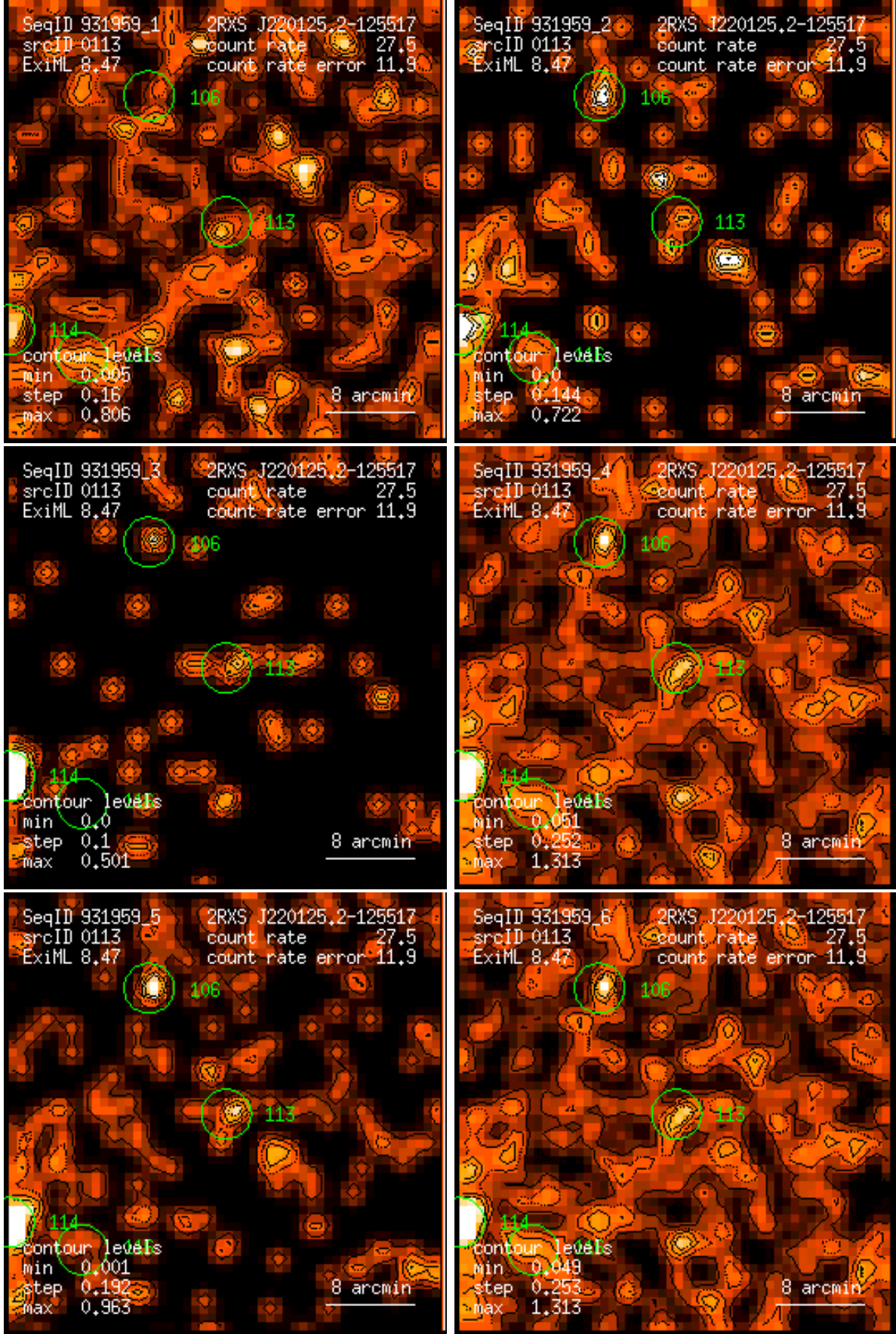
Figure 113: RASS 931959: detection 0113: band rate images, Gaussian filter: (1) PSPC channels 11 – 41, (2) 52 – 90, (3) 91 – 201, (4) 11 – 235, (5) 52 – 201, (6) 11 – 201. Broad band rates in counts/ks. Band rate contour levels in counts/ks/arcmin 2 .
