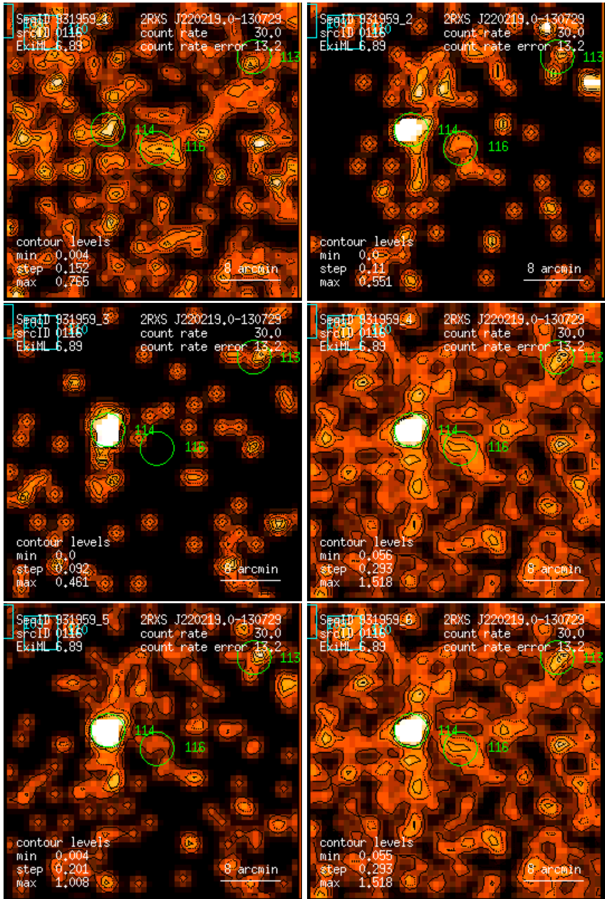
Figure 116: RASS 931959: detection 0116: band rate images, Gaussian filter: (1) PSPC channels 11 – 41, (2) 52 – 90, (3) 91 – 201, (4) 11 – 235, (5) 52 – 201, (6) 11 – 201. Broad band rates in counts/ks. Band rate contour levels in counts/ks/arcmin 2 .
