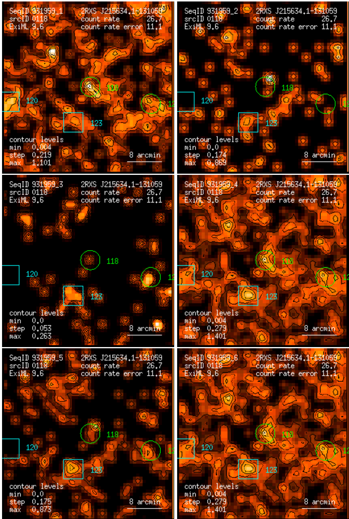
Figure 118: RASS 931959: detection 0118: band rate images, Gaussian filter: (1) PSPC channels 11 – 41, (2) 52 – 90, (3) 91 – 201, (4) 11 – 235, (5) 52 – 201, (6) 11 – 201. Broad band rates in counts/ks. Band rate contour levels in counts/ks/arcmin 2 .
