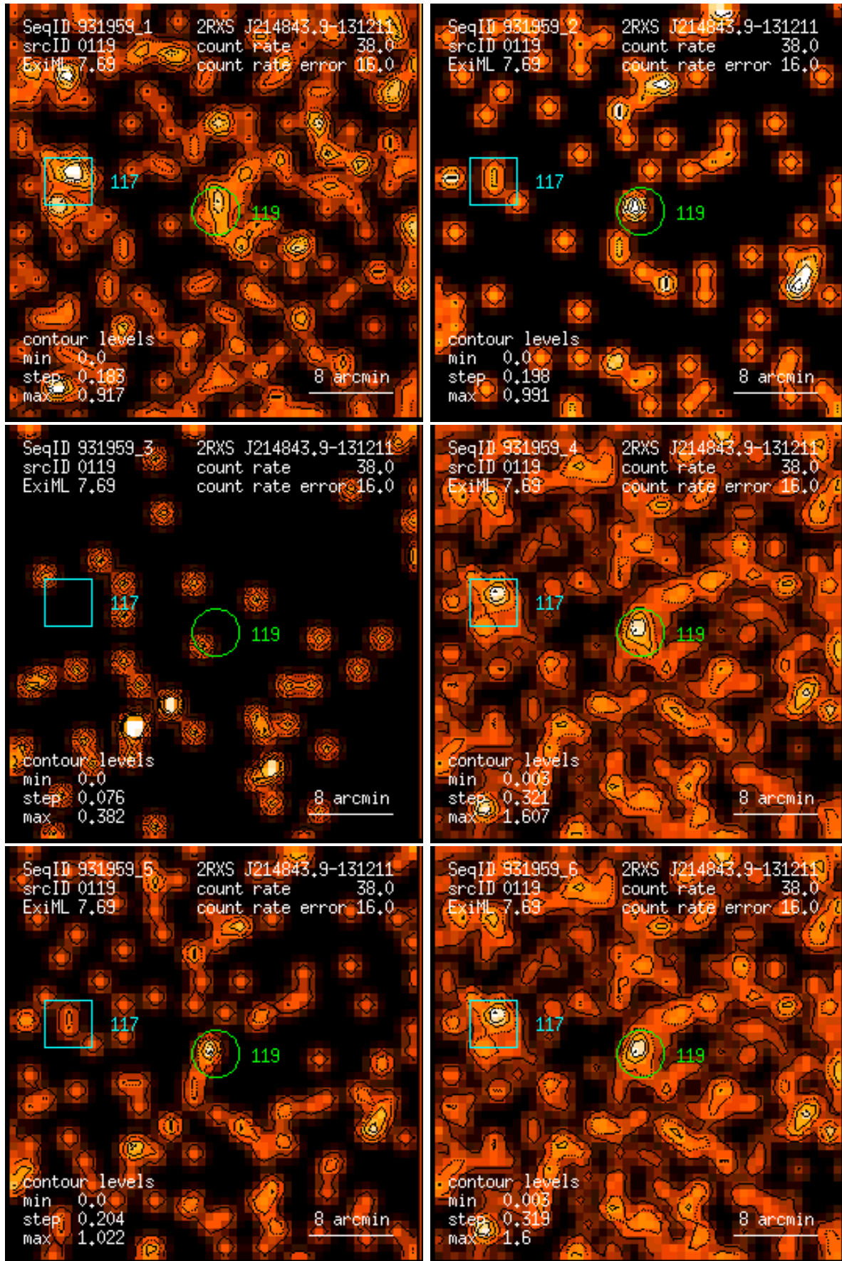
Figure 119: RASS 931959: detection 0119: band rate images, Gaussian filter: (1) PSPC channels 11 – 41, (2) 52 – 90, (3) 91 – 201, (4) 11 – 235, (5) 52 – 201, (6) 11 – 201. Broad band rates in counts/ks. Band rate contour levels in counts/ks/arcmin 2 .
