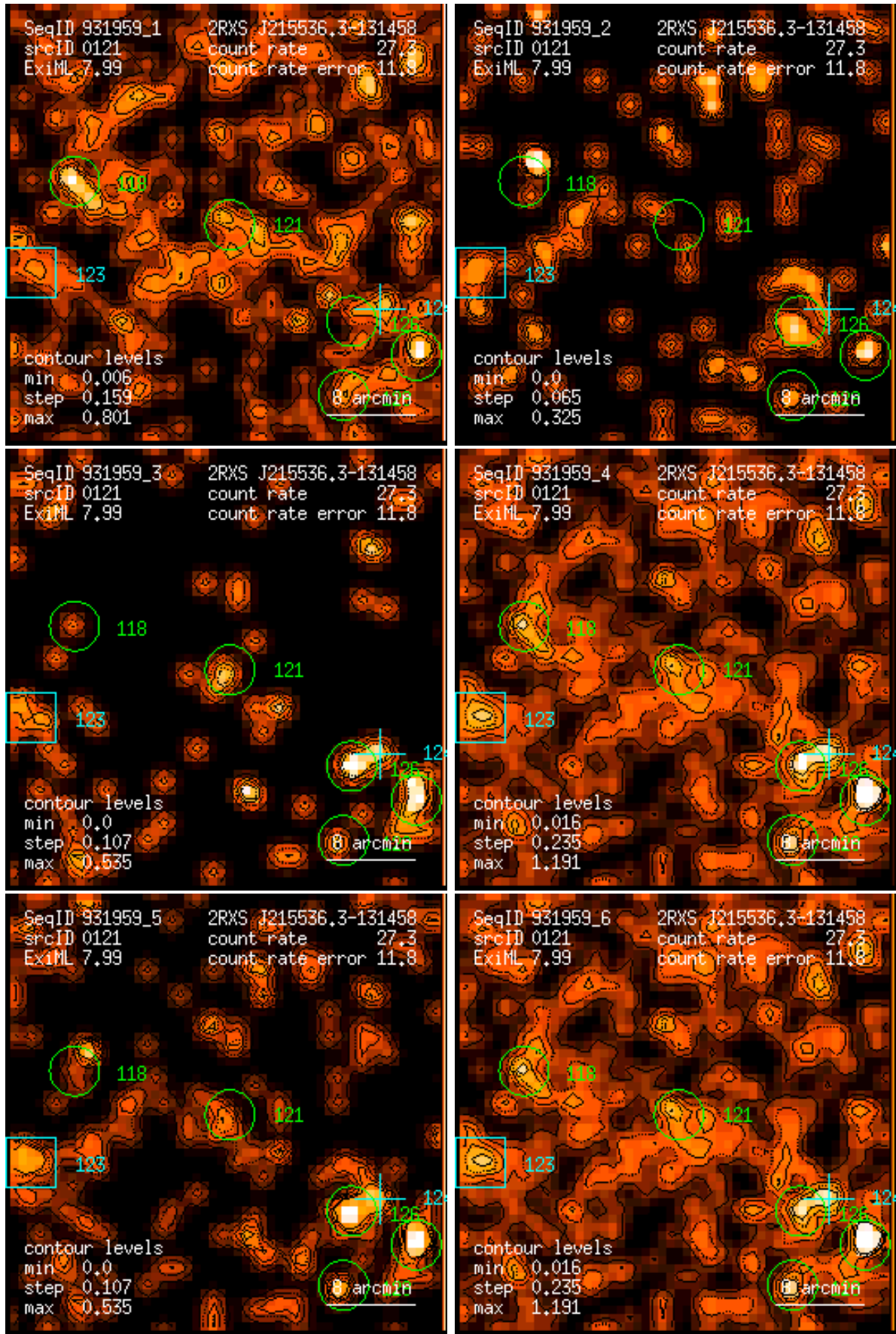
Figure 121: RASS 931959: detection 0121: band rate images, Gaussian filter: (1) PSPC channels 11 – 41, (2) 52 – 90, (3) 91 – 201, (4) 11 – 235, (5) 52 – 201, (6) 11 – 201. Broad band rates in counts/ks. Band rate contour levels in counts/ks/arcmin 2 .
