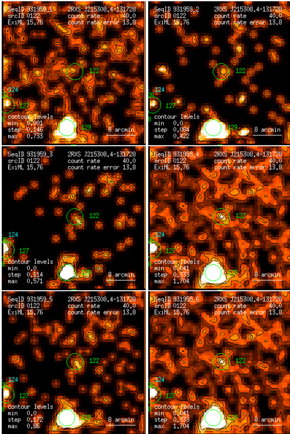
Figure 122: RASS 931959: detection 0122: band rate images, Gaussian filter: (1) PSPC channels 11 – 41, (2) 52 – 90, (3) 91 – 201, (4) 11 – 235, (5) 52 – 201, (6) 11 – 201. Broad band rates in counts/ks. Band rate contour levels in counts/ks/arcmin 2 .
