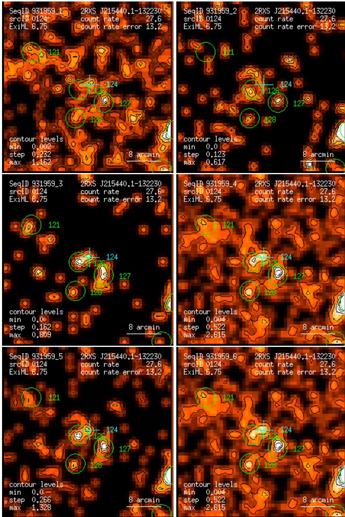
Figure 124: RASS 931959: detection 0124: band rate images, Gaussian filter: (1) PSPC channels 11 – 41, (2) 52 – 90, (3) 91 – 201, (4) 11 – 235, (5) 52 – 201, (6) 11 – 201. Broad band rates in counts/ks. Band rate contour levels in counts/ks/arcmin 2 .
