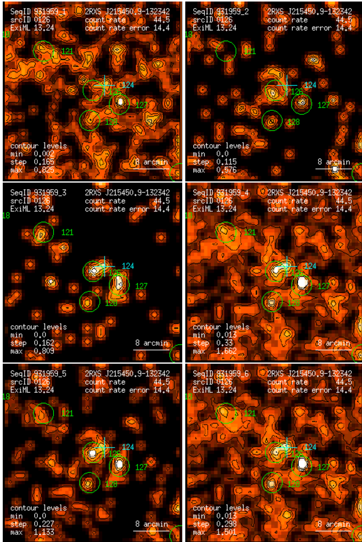
Figure 126: RASS 931959: detection 0126: band rate images, Gaussian filter: (1) PSPC channels 11 – 41, (2) 52 – 90, (3) 91 – 201, (4) 11 – 235, (5) 52 – 201, (6) 11 – 201. Broad band rates in counts/ks. Band rate contour levels in counts/ks/arcmin 2 .
