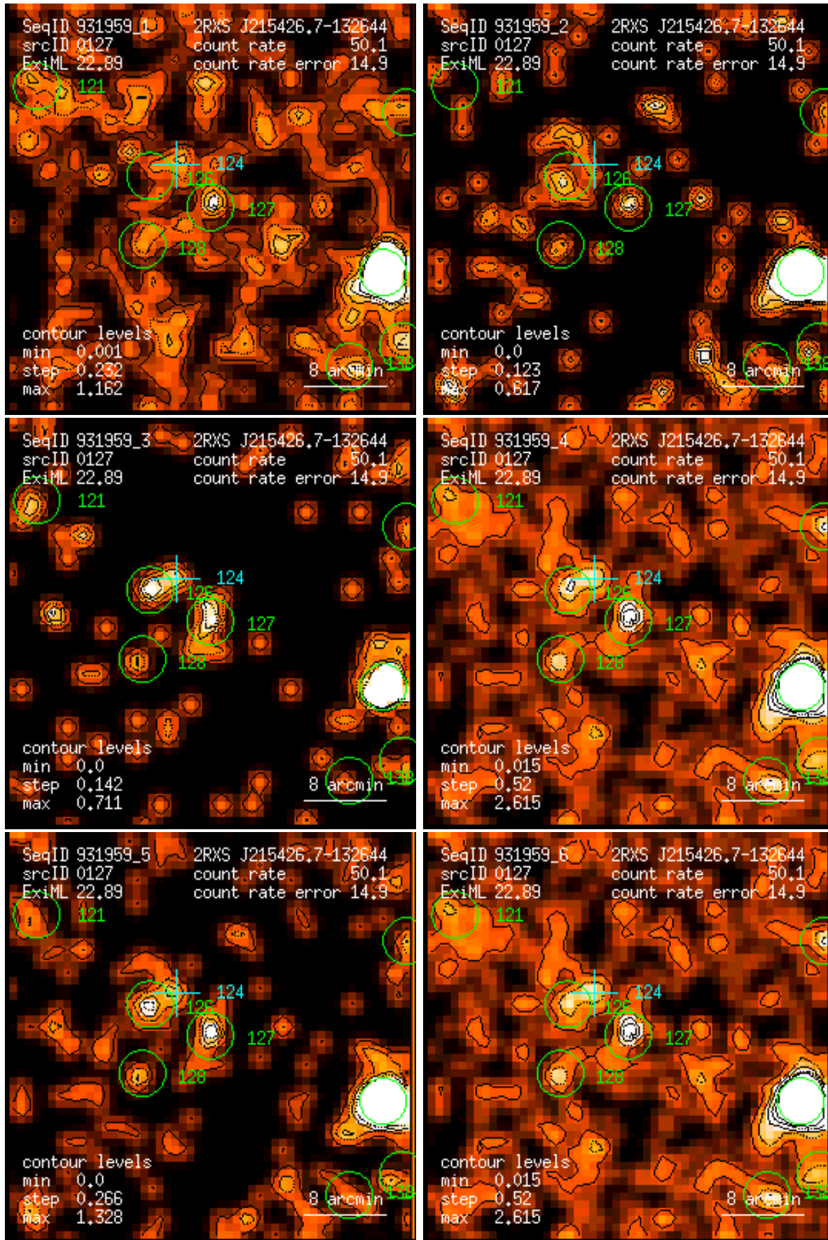
Figure 127: RASS 931959: detection 0127: band rate images, Gaussian filter: (1) PSPC channels 11 – 41, (2) 52 – 90, (3) 91 – 201, (4) 11 – 235, (5) 52 – 201, (6) 11 – 201. Broad band rates in counts/ks. Band rate contour levels in counts/ks/arcmin 2 .
