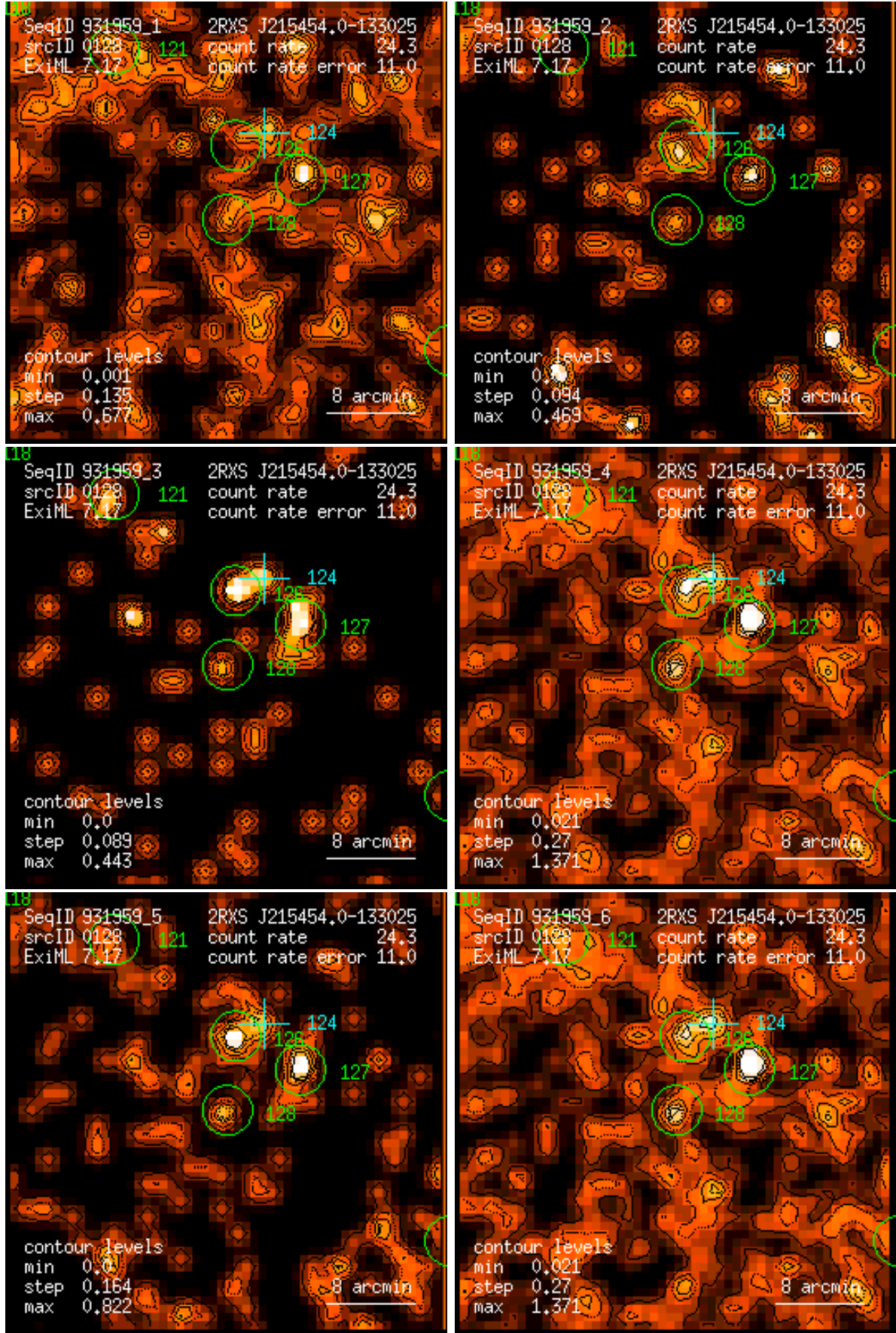
Figure 128: RASS 931959: detection 0128: band rate images, Gaussian filter: (1) PSPC channels 11 – 41, (2) 52 – 90, (3) 91 – 201, (4) 11 – 235, (5) 52 – 201, (6) 11 – 201. Broad band rates in counts/ks. Band rate contour levels in counts/ks/arcmin 2 .
