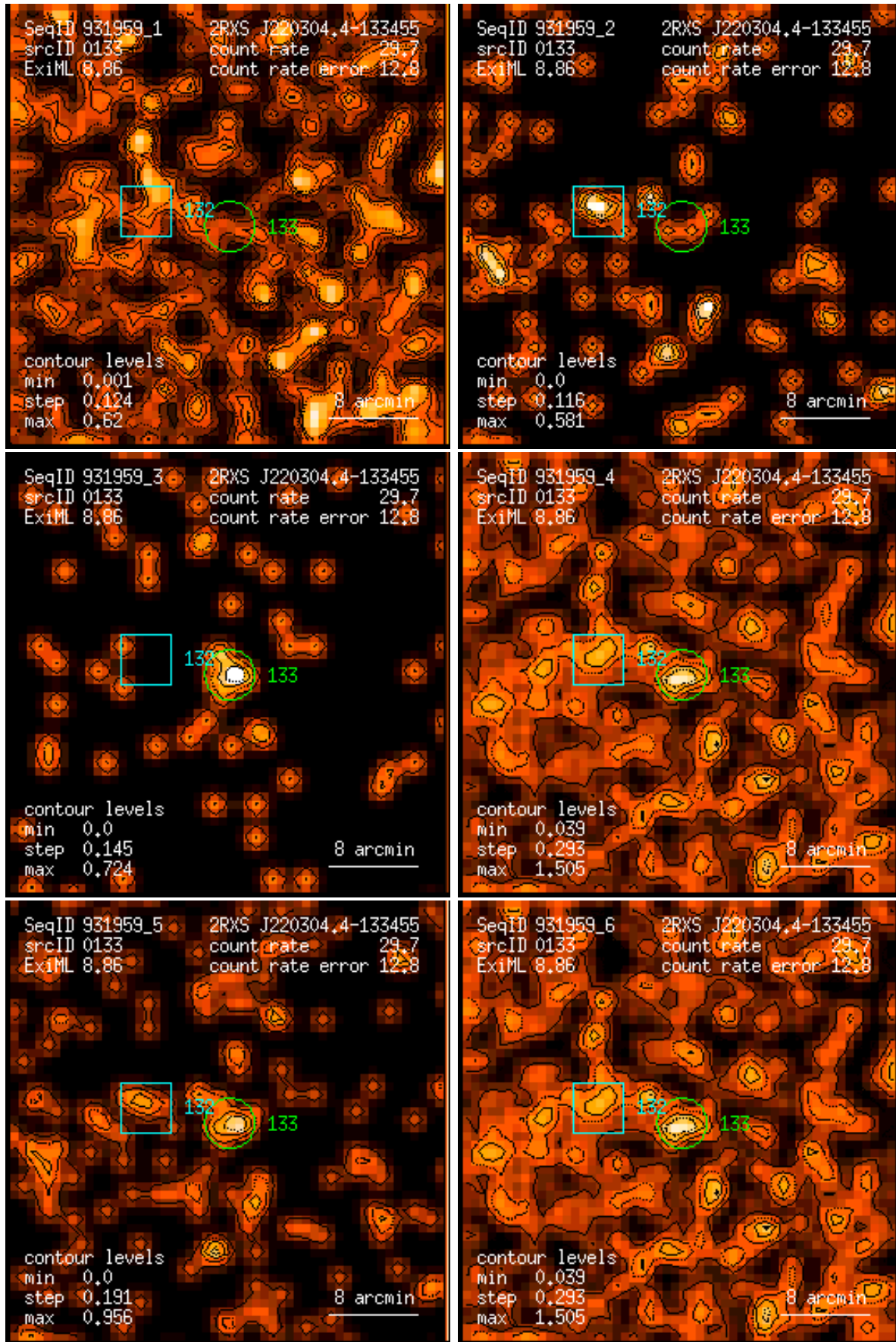
Figure 133: RASS 931959: detection 0133: band rate images, Gaussian filter: (1) PSPC channels 11 – 41, (2) 52 – 90, (3) 91 – 201, (4) 11 – 235, (5) 52 – 201, (6) 11 – 201. Broad band rates in counts/ks. Band rate contour levels in counts/ks/arcmin 2 .
