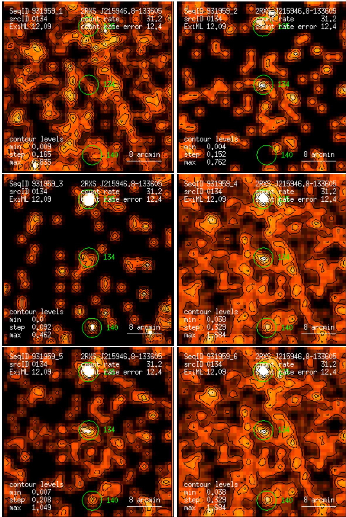
Figure 134: RASS 931959: detection 0134: band rate images, Gaussian filter: (1) PSPC channels 11 – 41, (2) 52 – 90, (3) 91 – 201, (4) 11 – 235, (5) 52 – 201, (6) 11 – 201. Broad band rates in counts/ks. Band rate contour levels in counts/ks/arcmin 2 .
