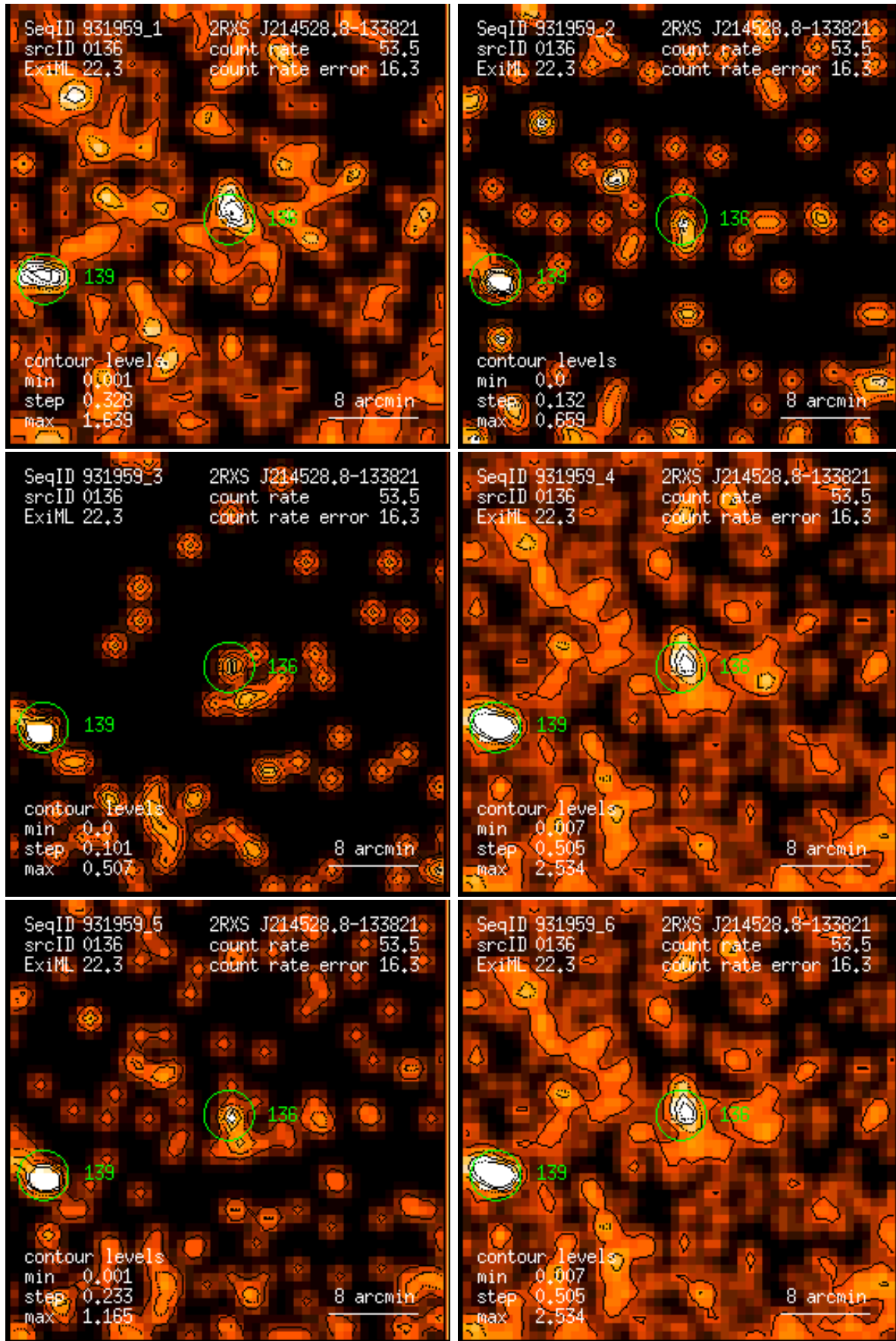
Figure 136: RASS 931959: detection 0136: band rate images, Gaussian filter: (1) PSPC channels 11 – 41, (2) 52 – 90, (3) 91 – 201, (4) 11 – 235, (5) 52 – 201, (6) 11 – 201. Broad band rates in counts/ks. Band rate contour levels in counts/ks/arcmin 2 .
